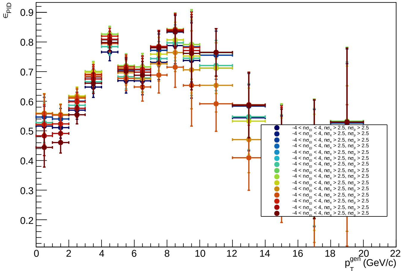
J/ψ PID Efficiency Comparison, LHC25b14
