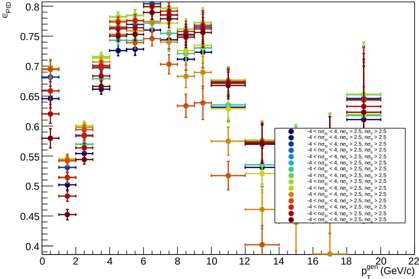
J/ψ PID Efficiency Comparison, LHC25b16
