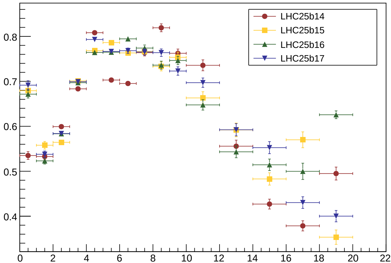
J/\psi Avg. PID-Efficiency Comparison between datasets
