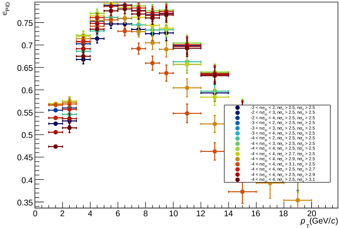
Non-Prompt-J/ \psi PID Efficiency Comparison, LHC25b14
