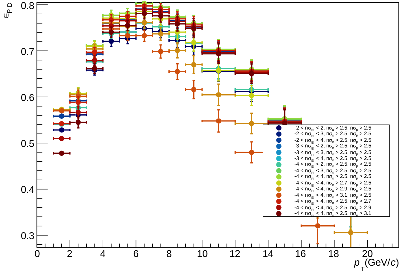
Non-Prompt-J/ \psi PID Efficiency Comparison, LHC25b16
