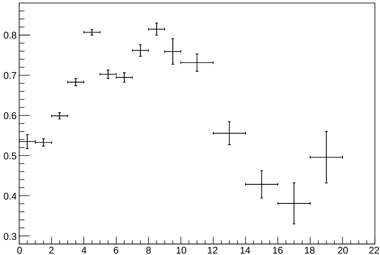
J/\psi PID Efficiency Comparison, LHC25b14
