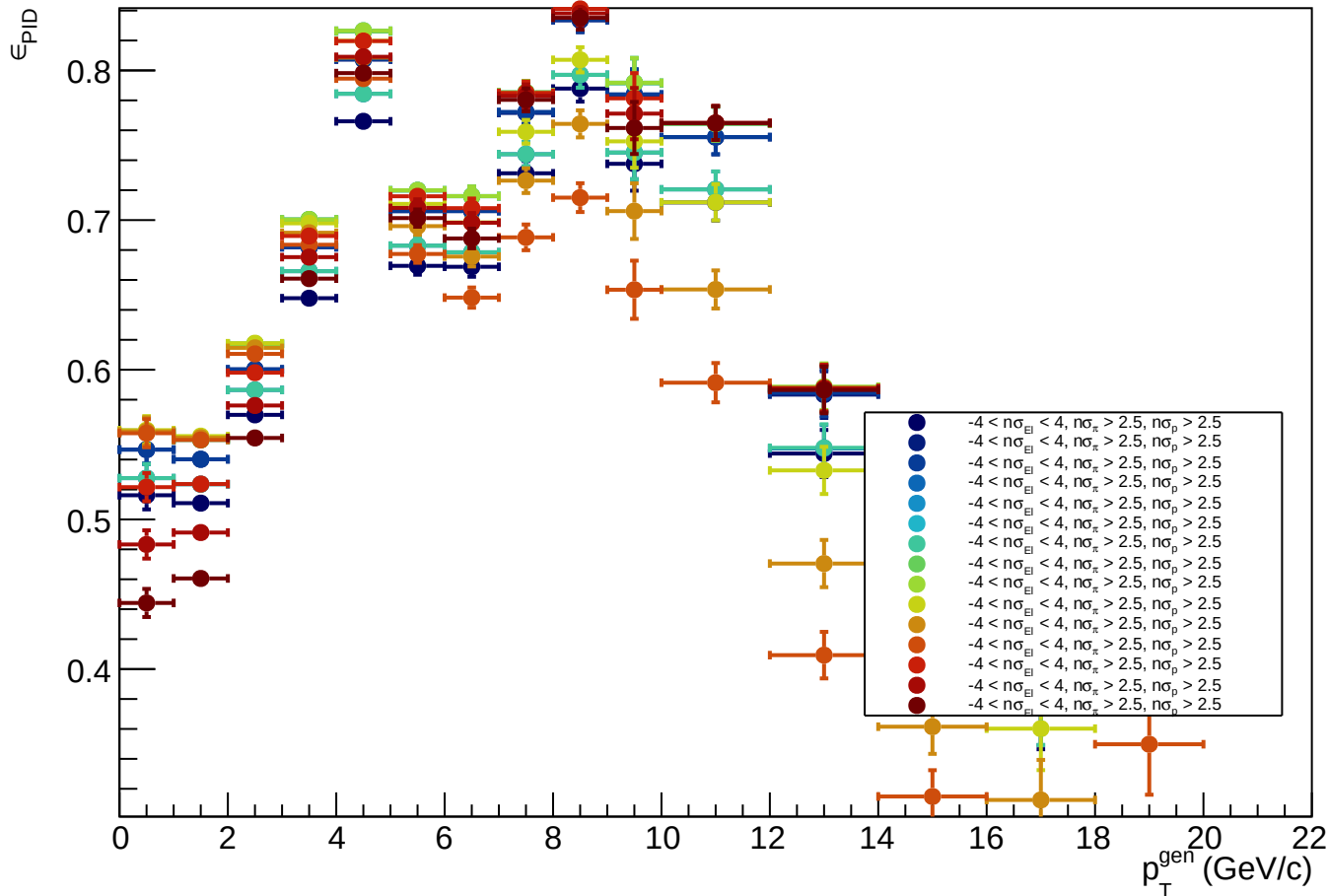
J/ψ PID Efficiency Comparison
