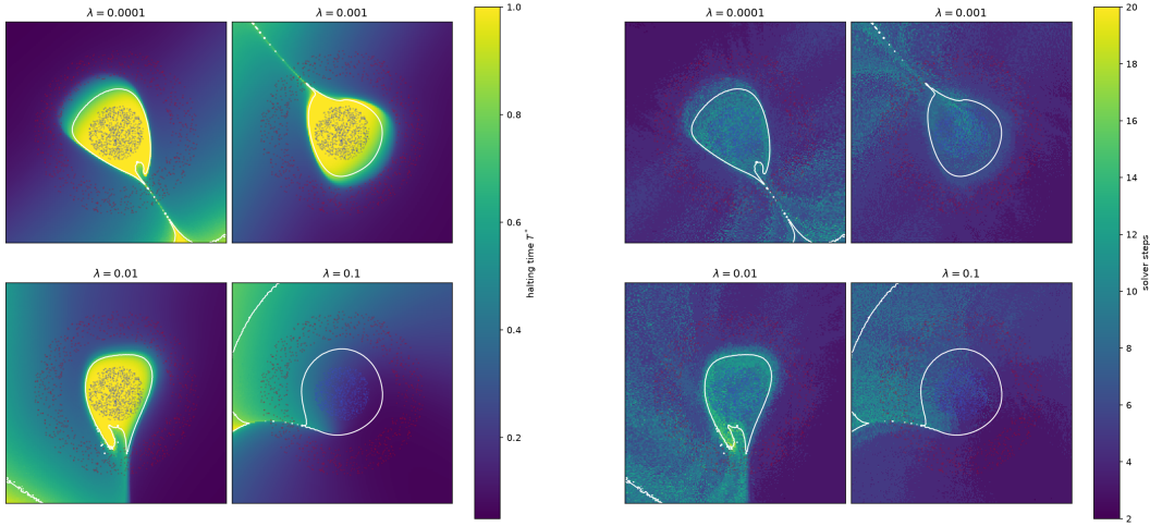
Figure 3: Left: T^* heatmap for the inputs of g^{(2)} . Right: Solver steps heatmap for the inputs of g^{(2)} . The best model (decided by score, tie-broken by loss) of each \lambda over the 10 runs was used. The decision boundary is drawn in white.
