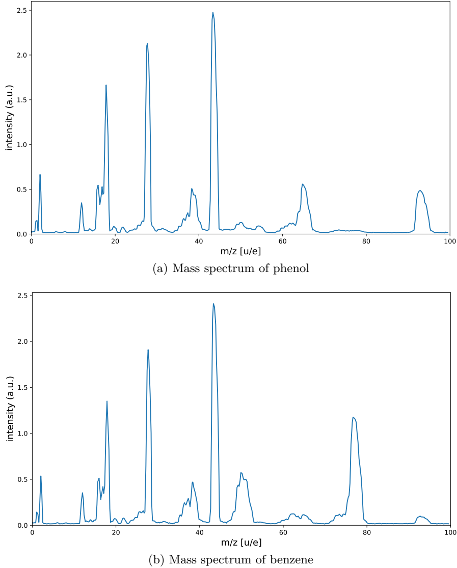
Figure 5: Mass spectra of benzene and phenol recorded using the QMS in the UHV chamber.
