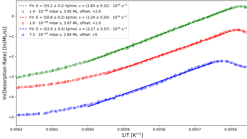
Figure 11: Menzel-Schlichting plot [6] for the multilayer of phenol on Ag(111). The desorption energy is calculated from the slope and the pre-exponential factor is calculated from the intercept of the Menzel-Schlichting plot.
