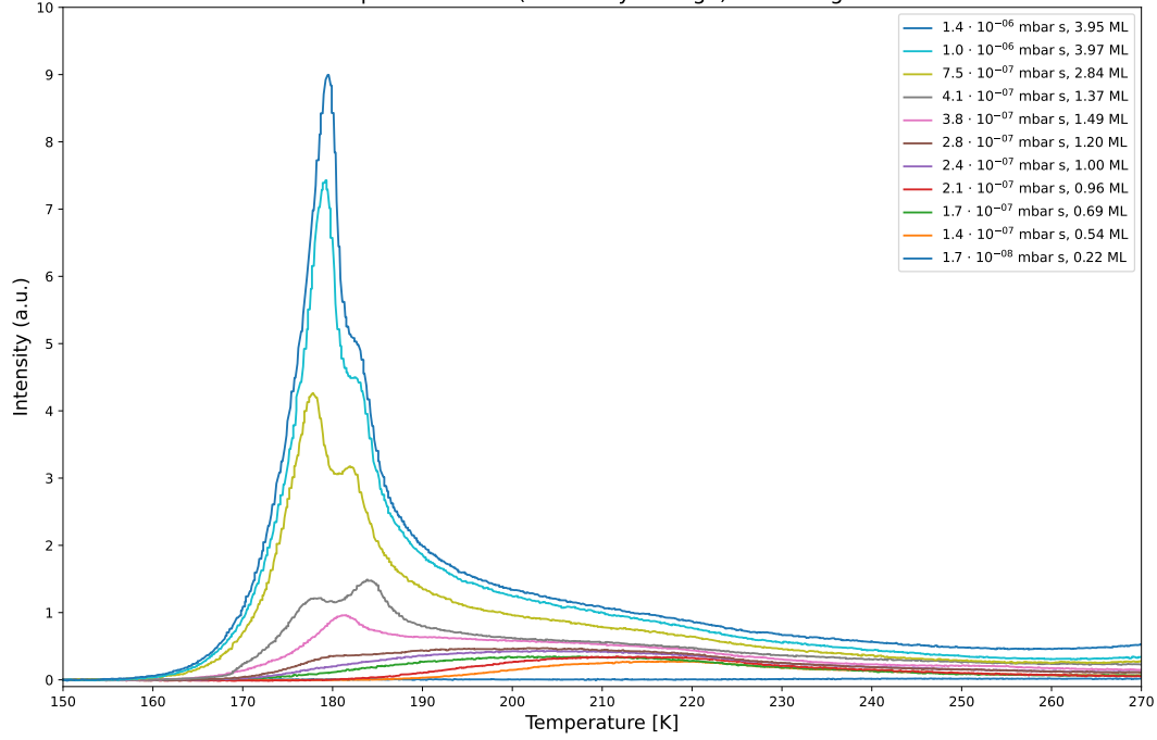
Figure 6: TDS spectrum of phenol on Ag(111) with different coverages between 0.22 and 3.95 ML.
