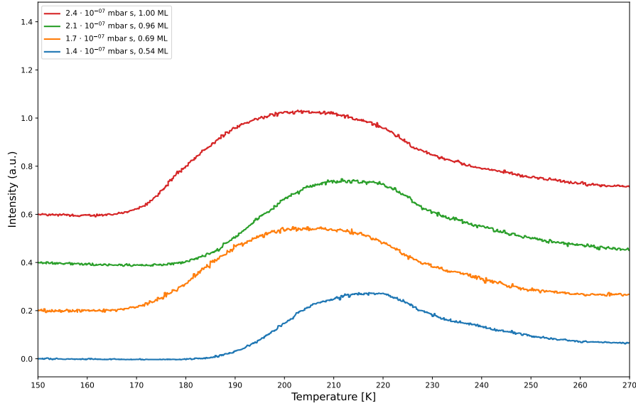
Figure 12: TDS spectra for the monolayer of phenol on Ag(111) with coverages below 1 ML with an offset of 0.2 between each spectrum.
