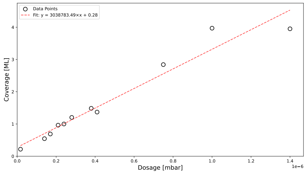
Figure 9: Coverage as a function of dosage for phenol on Ag(111). The coverage is calculated from the TDS spectra.
