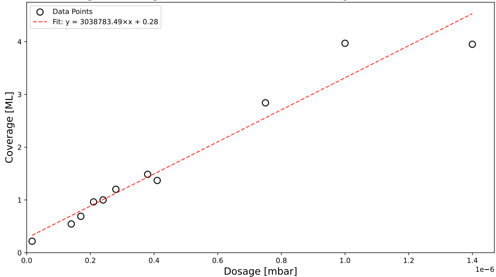
Coverage vs. Dosage for Phenol TPD (Reference Integral: 4.17\text{e}+01 = 1 \text{ ML} )
