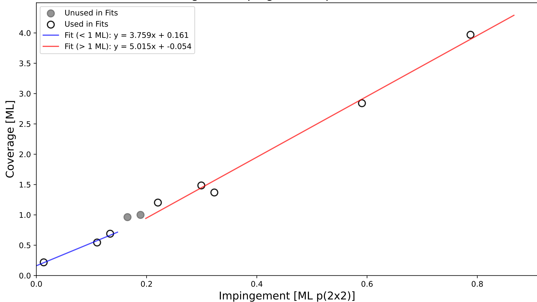
Coverage vs. Impingement - p(2x2) Structure
