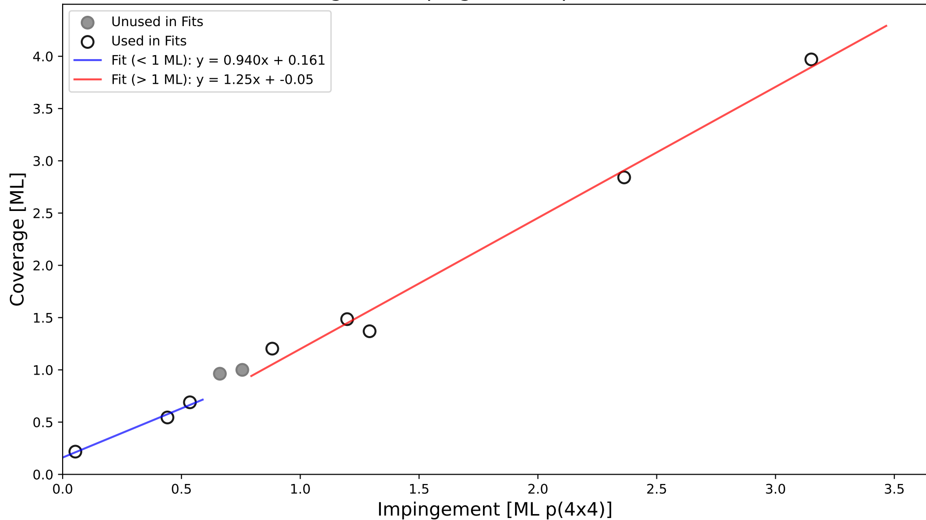
Coverage vs. Impingement - p(4x4) Structure
