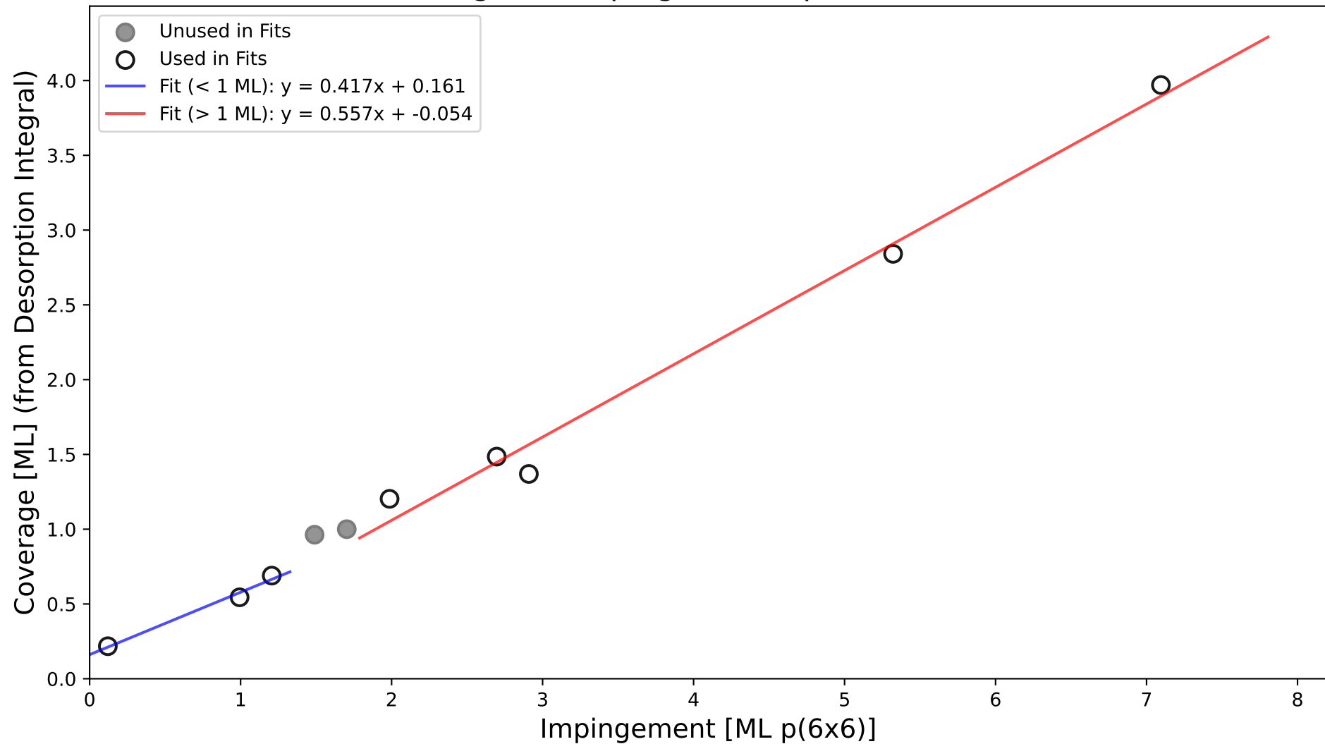
Coverage vs. Impingement - p(6x6) Structure
