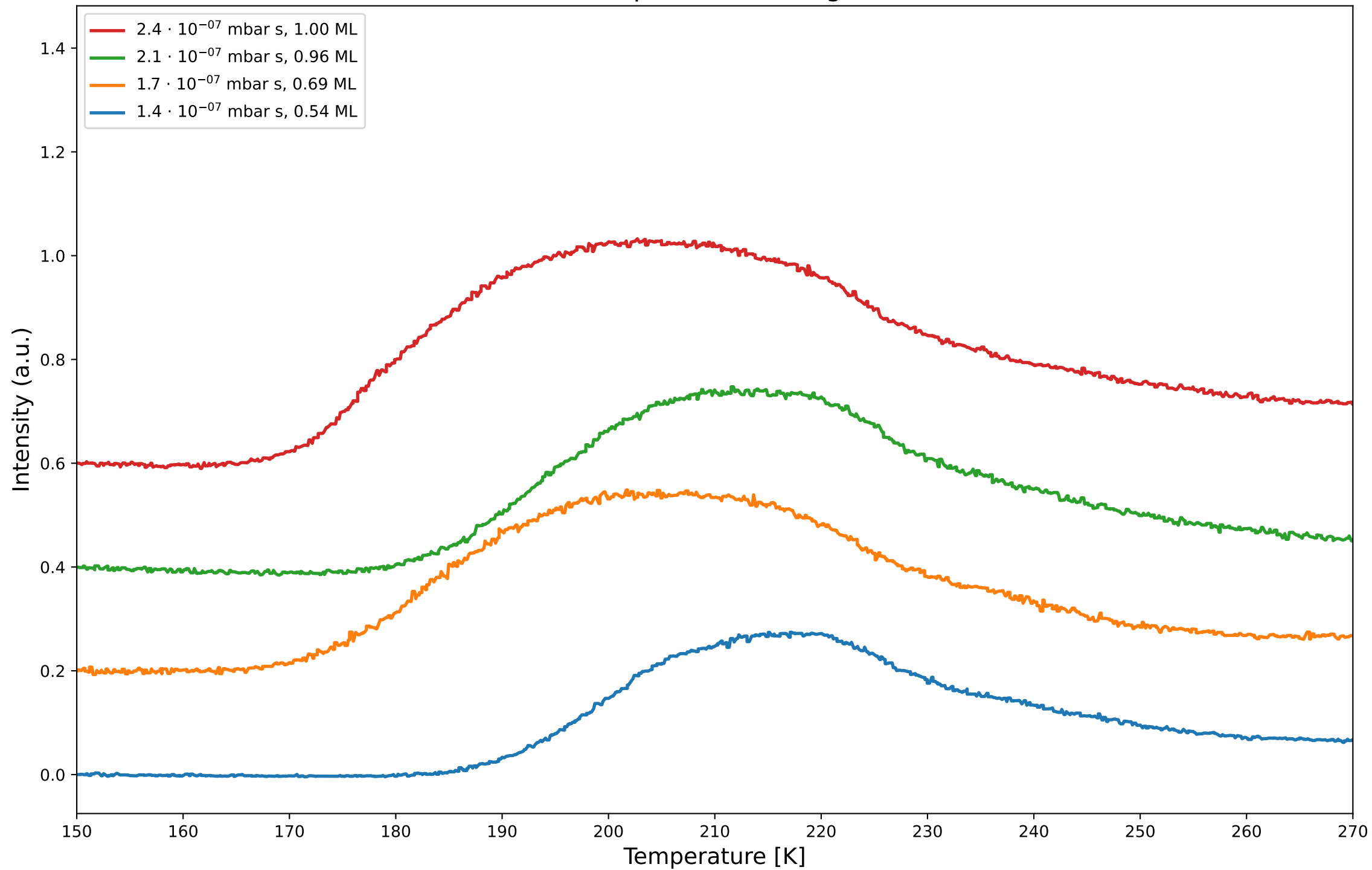
Phenol TPD Spectra (Coverage \leq 1 ML)
