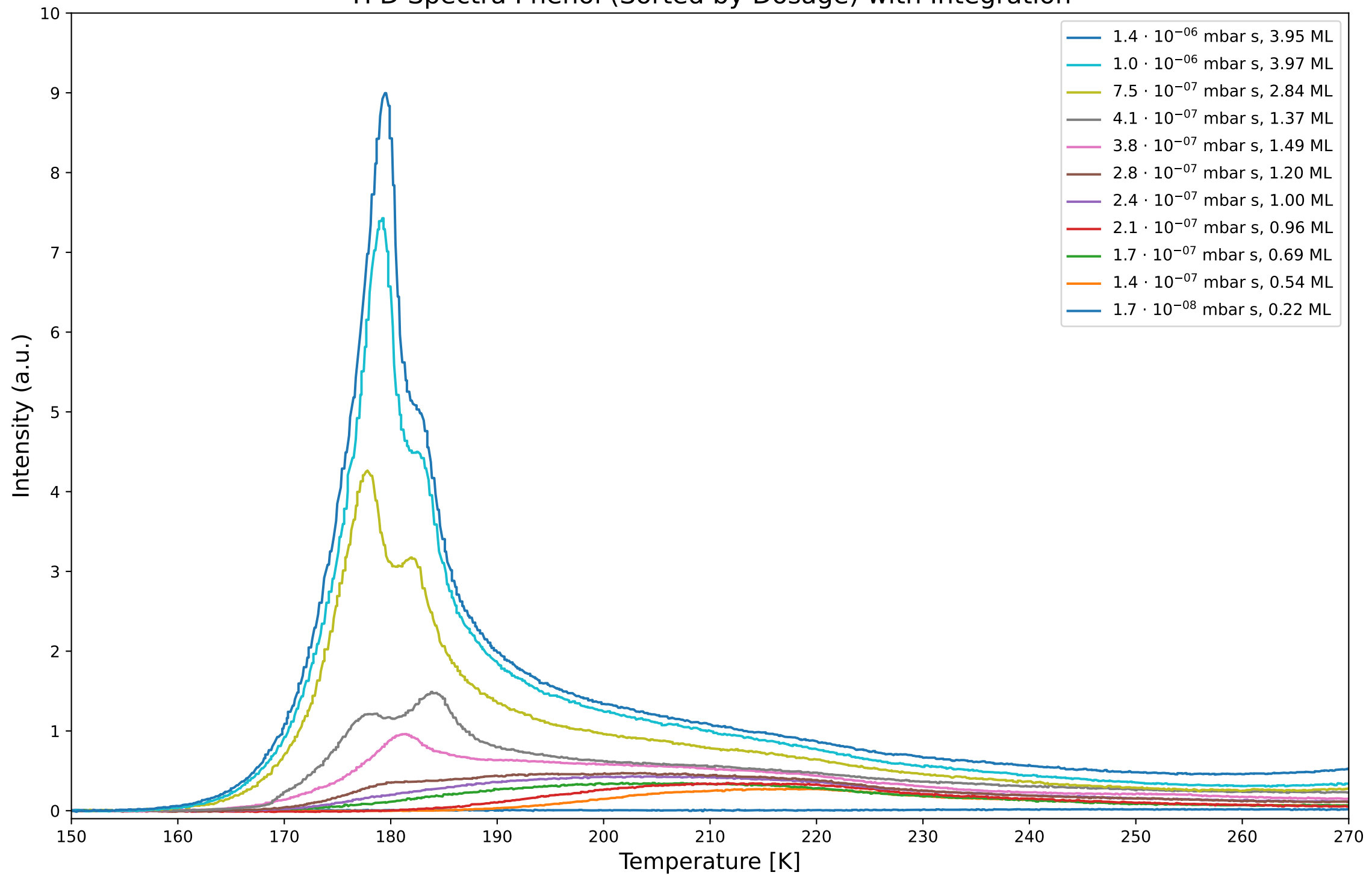
TPD Spectra Phenol (Sorted by Dosage) with Integration
