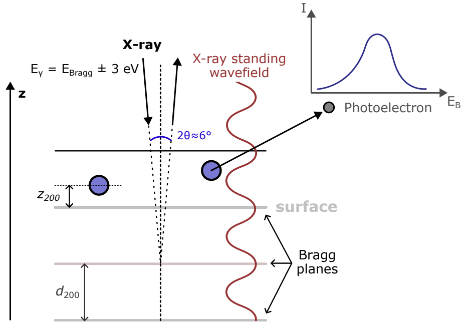
Figure 3.2: Schematic drawing of the principle of NIXSW. The image was adapted using reference [13].
