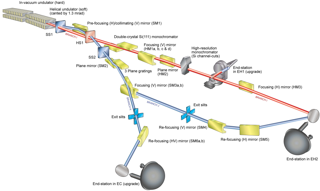
Figure 4.2: Schematic drawing of the I09 endstation of the Diamond Light Source in Didcot, UK. Picture taken from reference [23].
