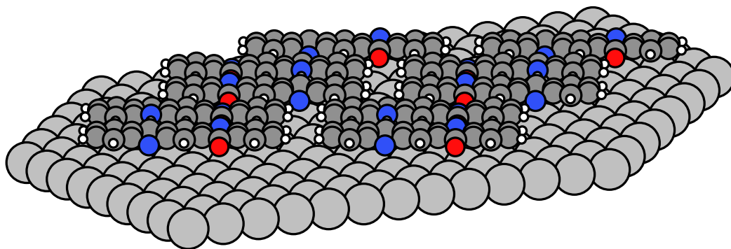
Figure 7.5: Long side view of the revised structure model for the \beta -phase of QA on the Ag(100) surface. The underlying Ag atoms at the corners of Figure 7.4 are deleted for better visibility.
