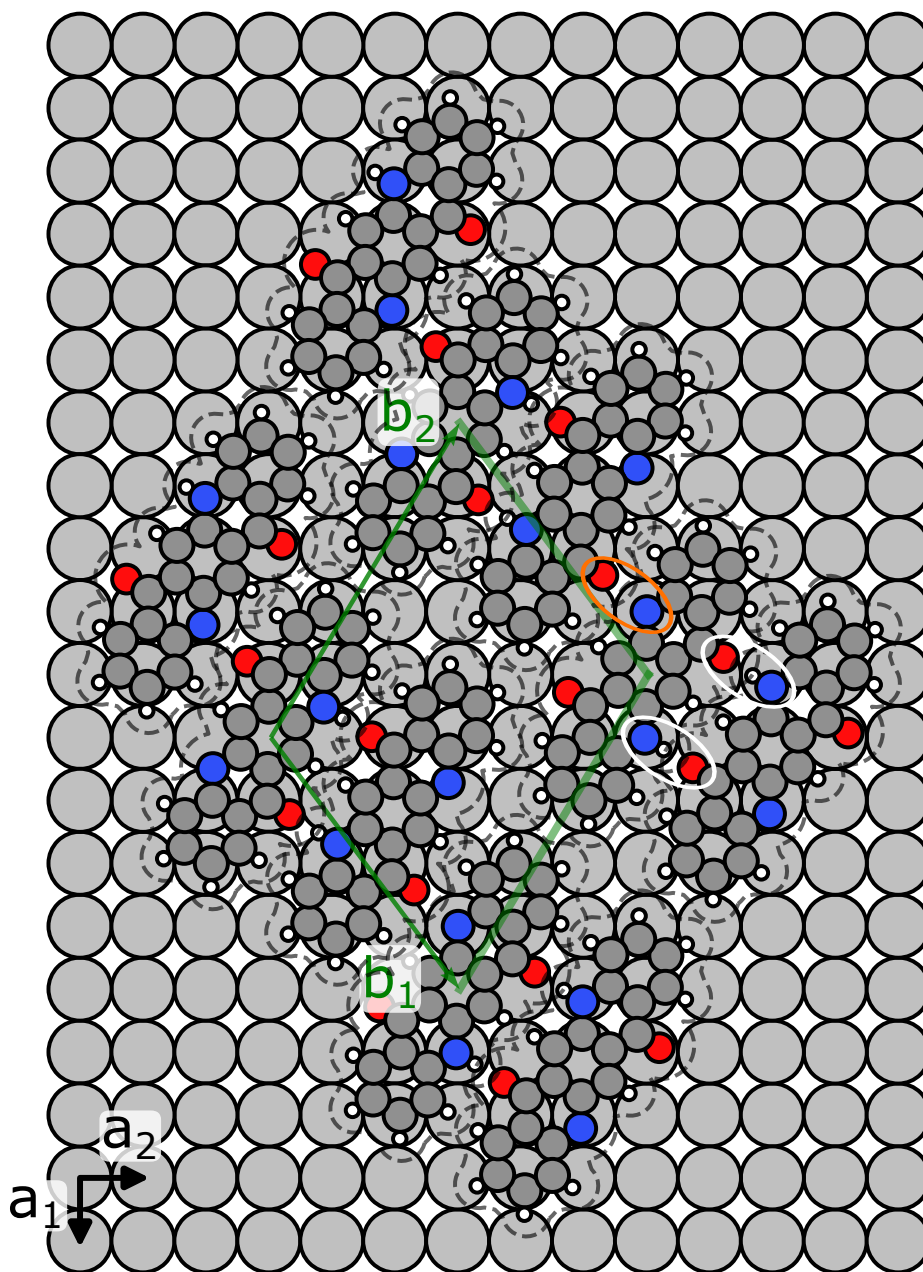
Figure 7.4: Top view of the structure model for the \beta -phase of QA on the Ag(100) surface. The hydrogen bonds between the O1 and N1 components are marked with white ellipses, while the missing hydrogen bond due to deprotonation between the O2 and N2 component is marked with an orange ellipse. The van der Waals radii of the atoms are shown as dashed grey lines. The unit cell is indicated by the green rectangle with the corresponding unit cell vectors \mathbf{b}_1 and \mathbf{b}_2 and is based on reference [1].
