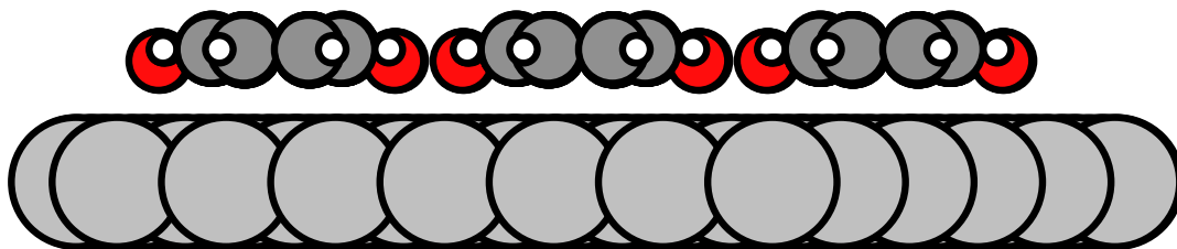
Figure 7.3: Short side view of the revised structure model for the \alpha -phase of QA on the Ag(100) surface.
