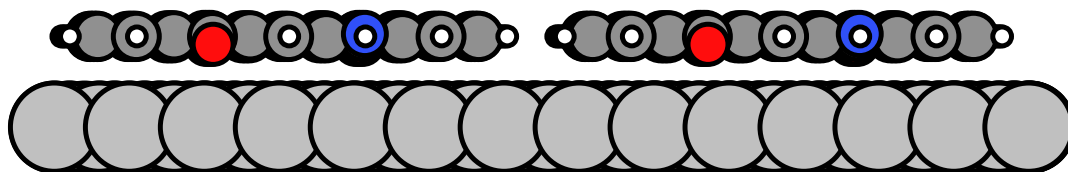
Figure 7.2: Long side view of the revised structure model for the \alpha -phase of QA on the Ag(100) surface.
