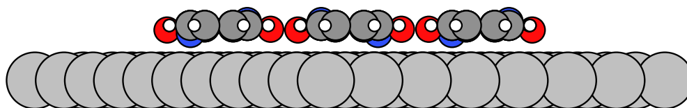
Figure 7.7: Short side view of the revised structure model for the \beta -phase of QA on the Ag(100) surface. The two QA molecules on the left are one dimer and form two hydrogen bonds, while the QA molecule on the right is part of the neighboring dimer without hydrogen bonds to the shown QA molecule.
