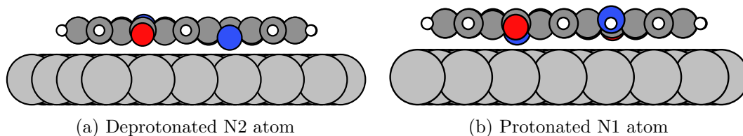
Figure 7.6: Long side views of the revised structure model for the \beta -phase of QA on the Ag(100) surface. The left image shows the side of the deprotonated N2 component, while the right image shows the side of the N1 component.
