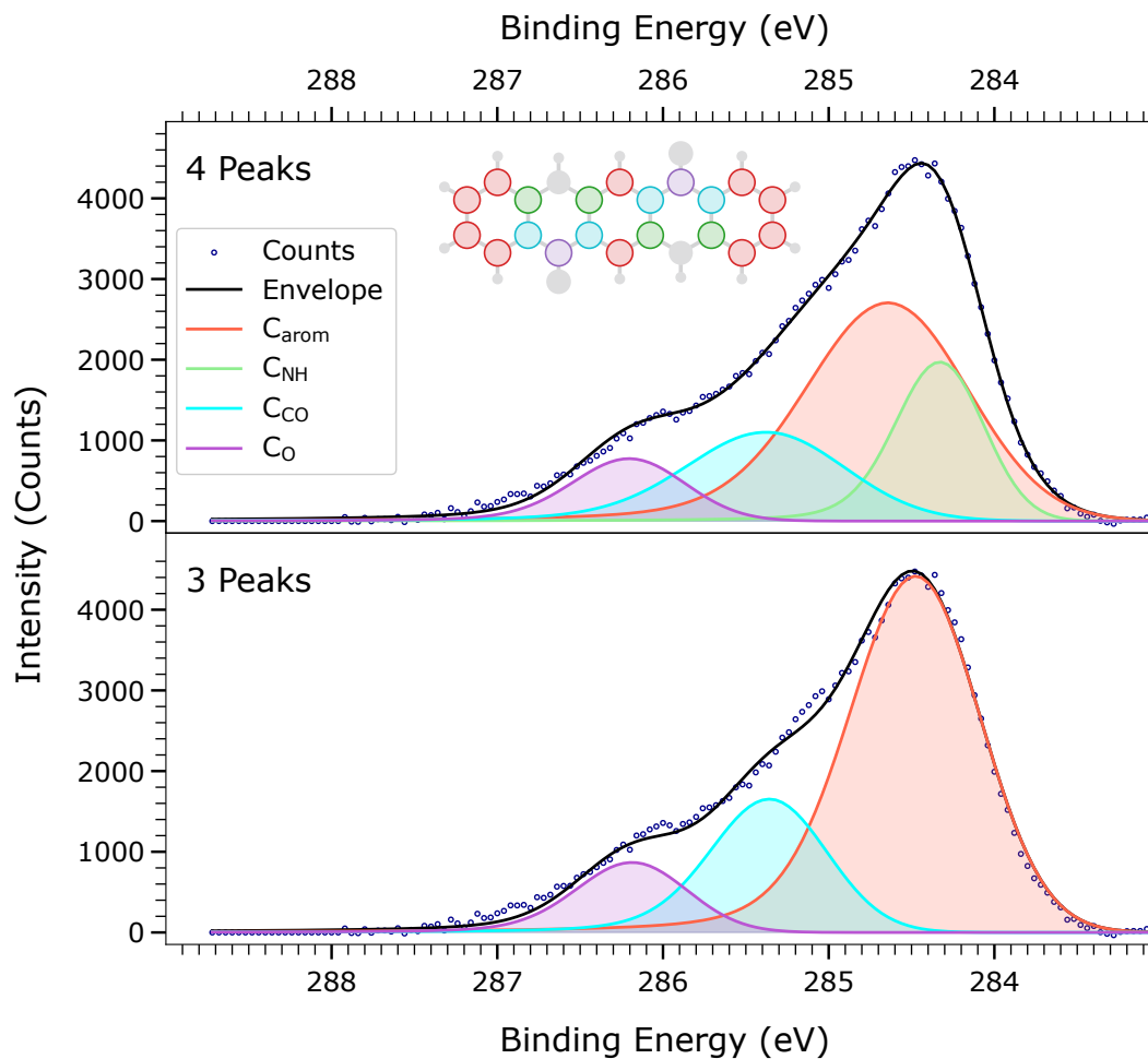
Figure 5.2: Comparison of the C1s XPS spectra of QA on the Ag(100) surface in the \beta -phase with 4 and 3 peaks fitted. The figure contains the counts (blue circles), C arom (red), C NH (green), C CO (lightblue), C O (purple) and the resulting envelope (black). The C NH peak is omitted in the fit with 3 peaks. The used fit parameters are summarized in Table 5.2.
