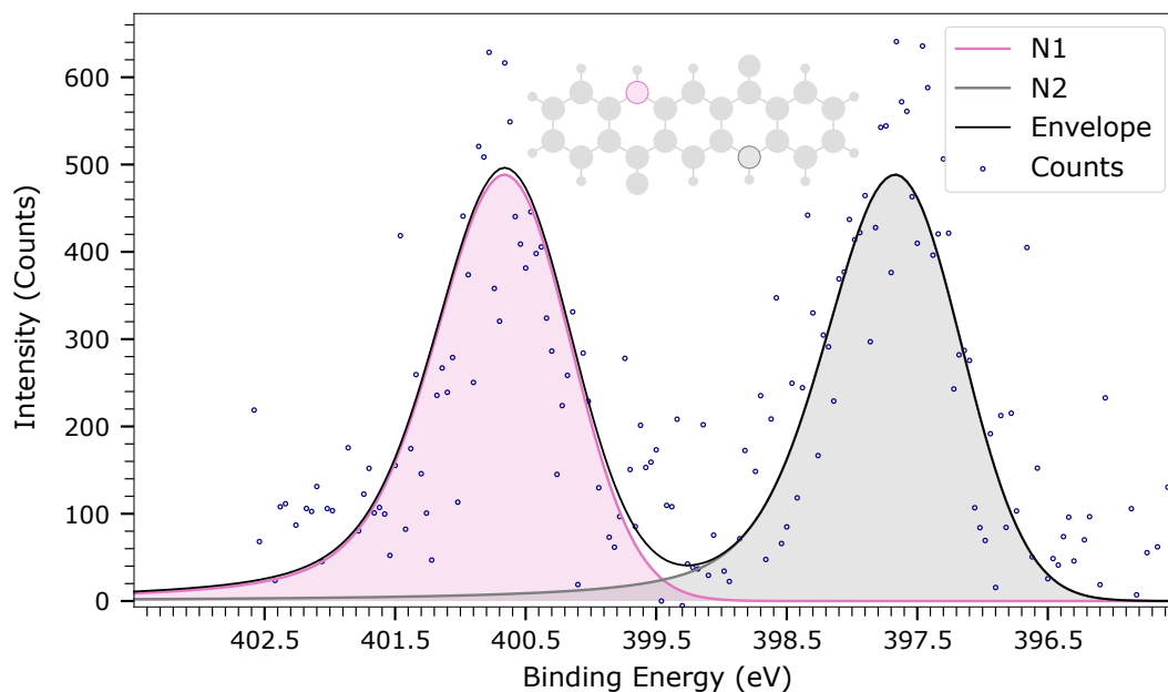
Figure 5.10: N1s XPS spectra of a damaged QA layer on the Ag(100) surface.
