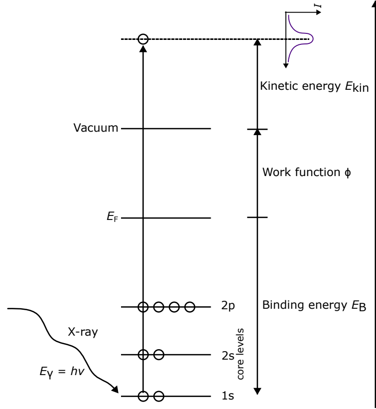
Figure 3.1: Schematic drawing of the photoemission process of an electron in the 1s orbital upon x-ray excitation. The image was adapted using reference [9].
