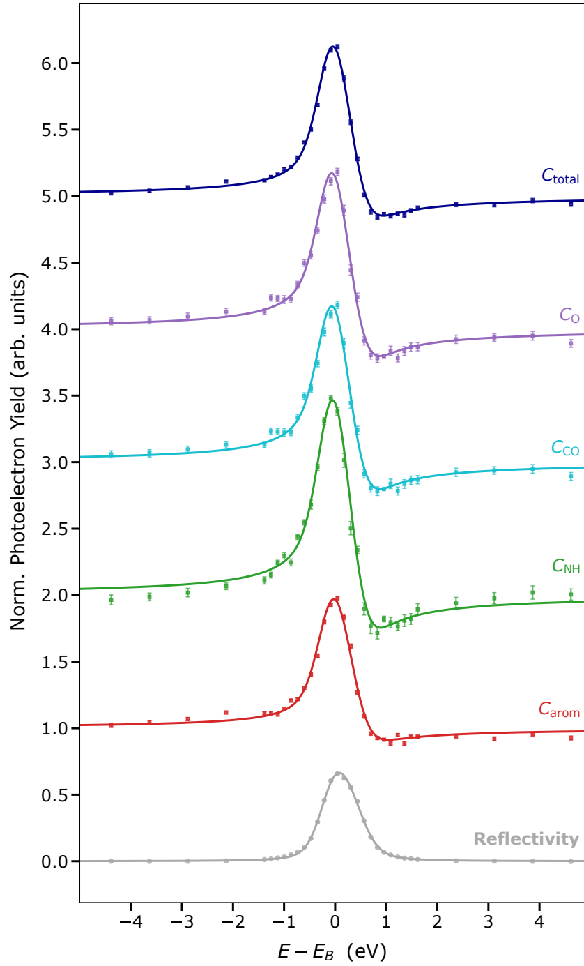
Figure 6.1: C1s NIXSW spectra of QA on the Ag(100) surface in the \alpha -phase. The sum of all components is shown at the top, followed by the individual components C_{\text{arom}} , C_{\text{NH}} , C_{\text{CO}} and C_{\text{O}} and the reflectivity at the bottom. For a better visibility, the different NIXSW spectra are shifted vertically by 1. The fit parameter from Table 5.1 were used for the individual XPS spectra.
