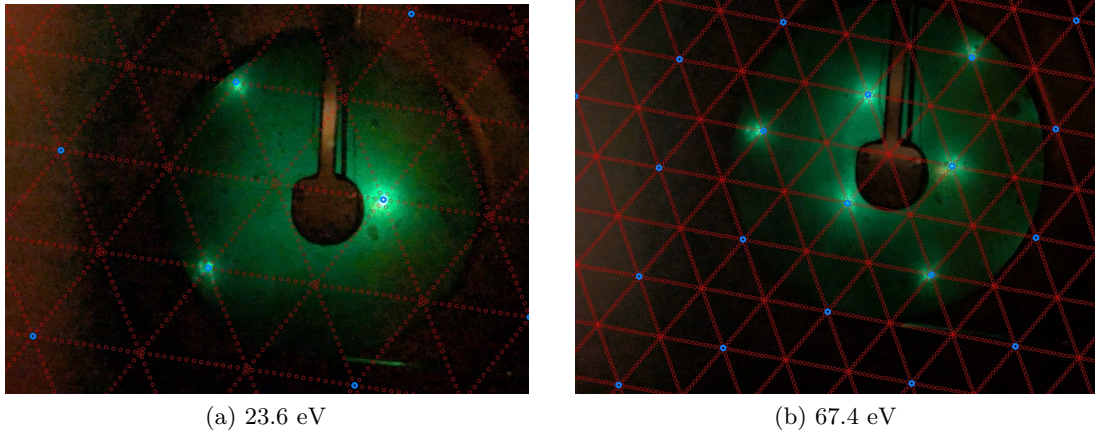
Figure 6: LEED patterns of the Au(111) surface at two different electron energies with the sample rotated showing the characteristic Au(111) reconstruction. The blue circles indicate the positions of the substrate spots. The reconstruction is indicated by the additional red circles in the pattern.
