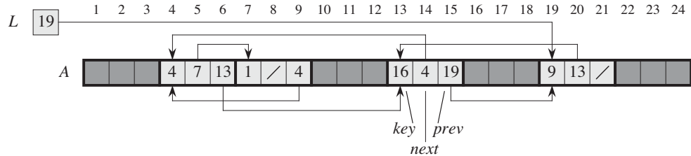
Figure 10.6 The linked list of Figures 10.3(a) and 10.5 represented in a single array A . Each list element is an object that occupies a contiguous subarray of length 3 within the array. The three attributes key , next , and prev correspond to the offsets 0, 1, and 2, respectively, within each object. A pointer to an object is the index of the first element of the object. Objects containing list elements are lightly shaded, and arrows show the list ordering.
