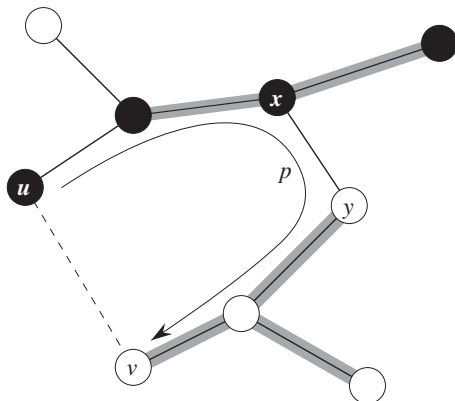
Figure 23.3 The proof of Theorem 23.1. Black vertices are in S , and white vertices are in V - S . The edges in the minimum spanning tree T are shown, but the edges in the graph G are not. The edges in A are shaded, and (u, v) is a light edge crossing the cut (S, V - S) . The edge (x, y) is an edge on the unique simple path p from u to v in T . To form a minimum spanning tree T' that contains (u, v) , remove the edge (x, y) from T and add the edge (u, v) .
