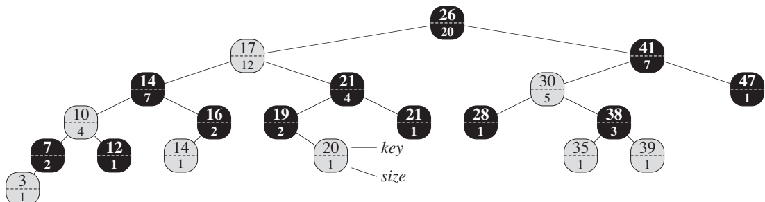
Figure 14.1 An order-statistic tree, which is an augmented red-black tree. Shaded nodes are red, and darkened nodes are black. In addition to its usual attributes, each node x has an attribute x.size , which is the number of nodes, other than the sentinel, in the subtree rooted at x .
