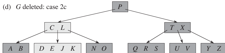
Figure 18.8 Deleting keys from a B-tree. The minimum degree for this B-tree is t = 3 , so a node (other than the root) cannot have fewer than 2 keys. Nodes that are modified are lightly shaded. (a) The B-tree of Figure 18.7(e). (b) Deletion of F . This is case 1: simple deletion from a leaf. (c) Deletion of M . This is case 2a: the predecessor L of M moves up to take M 's position. (d) Deletion of G . This is case 2c: we push G down to make node DEGJK and then delete G from this leaf (case 1).
