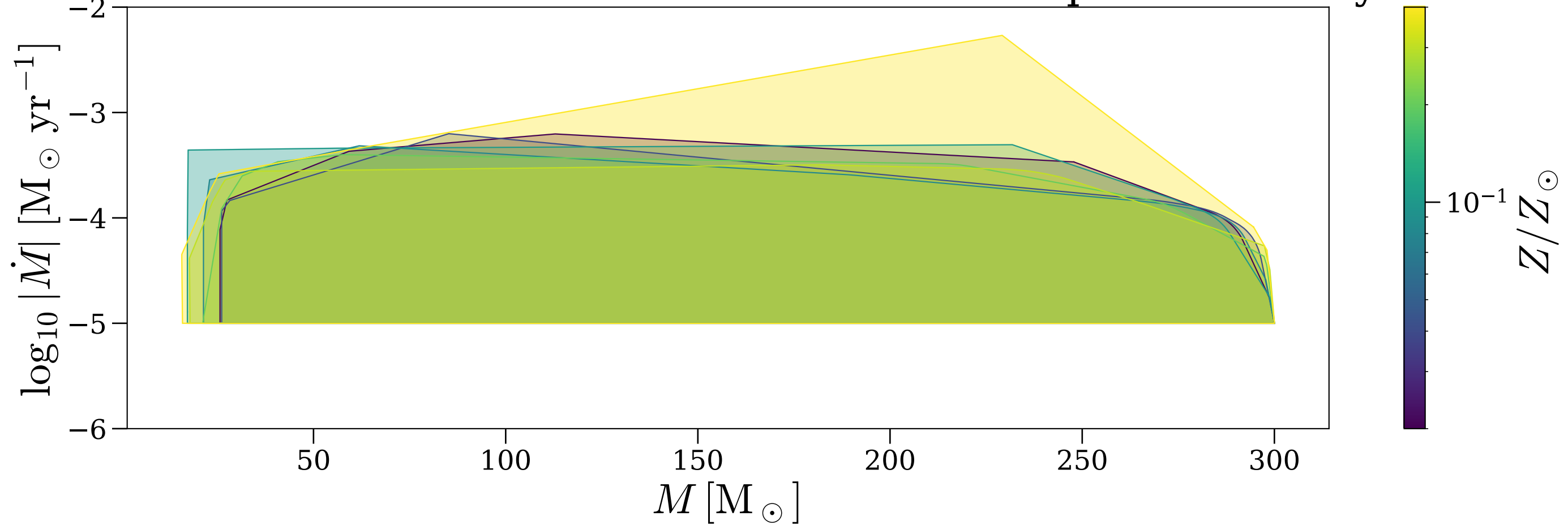
Mass-loss rate vs stellar mass — convex hulls per metallicity
