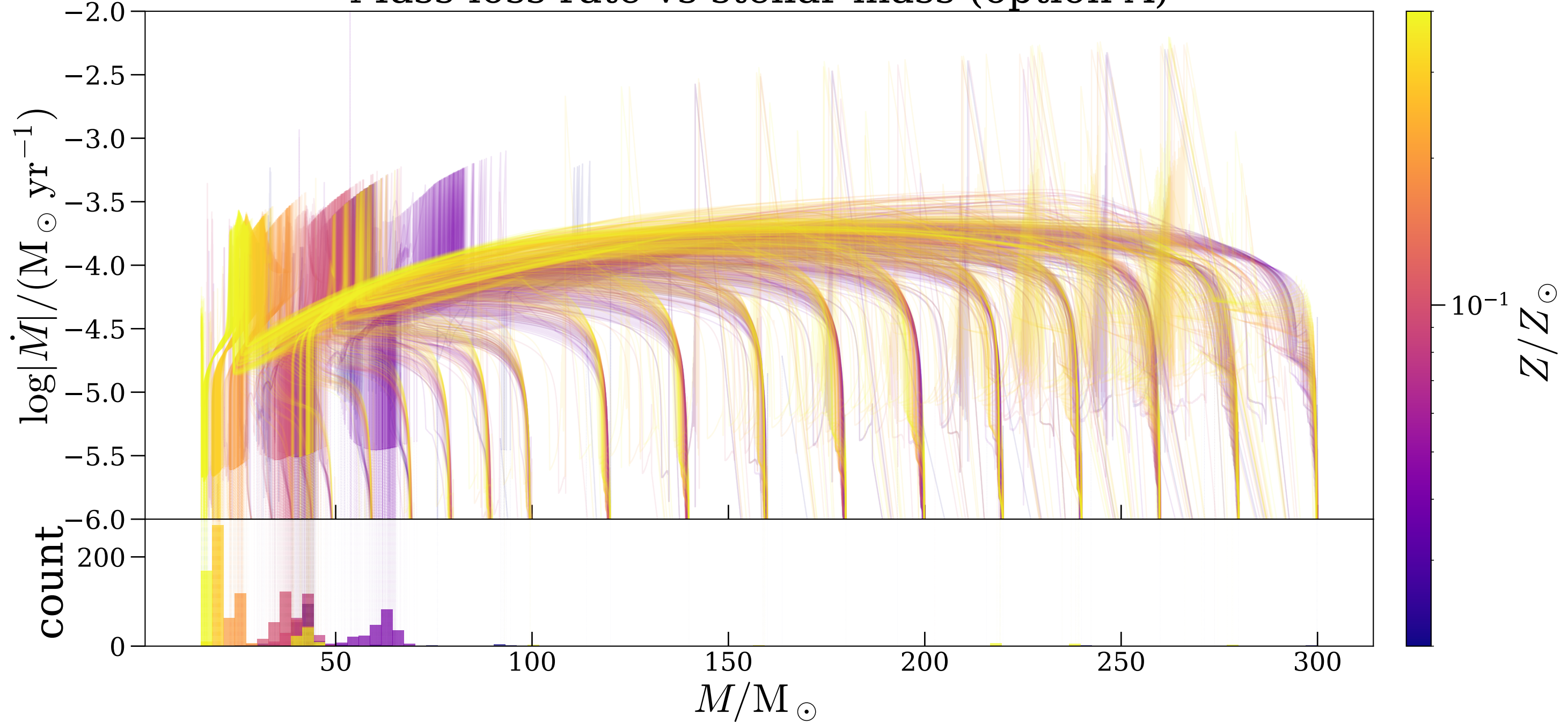
Mass-loss rate vs stellar mass (option A)
