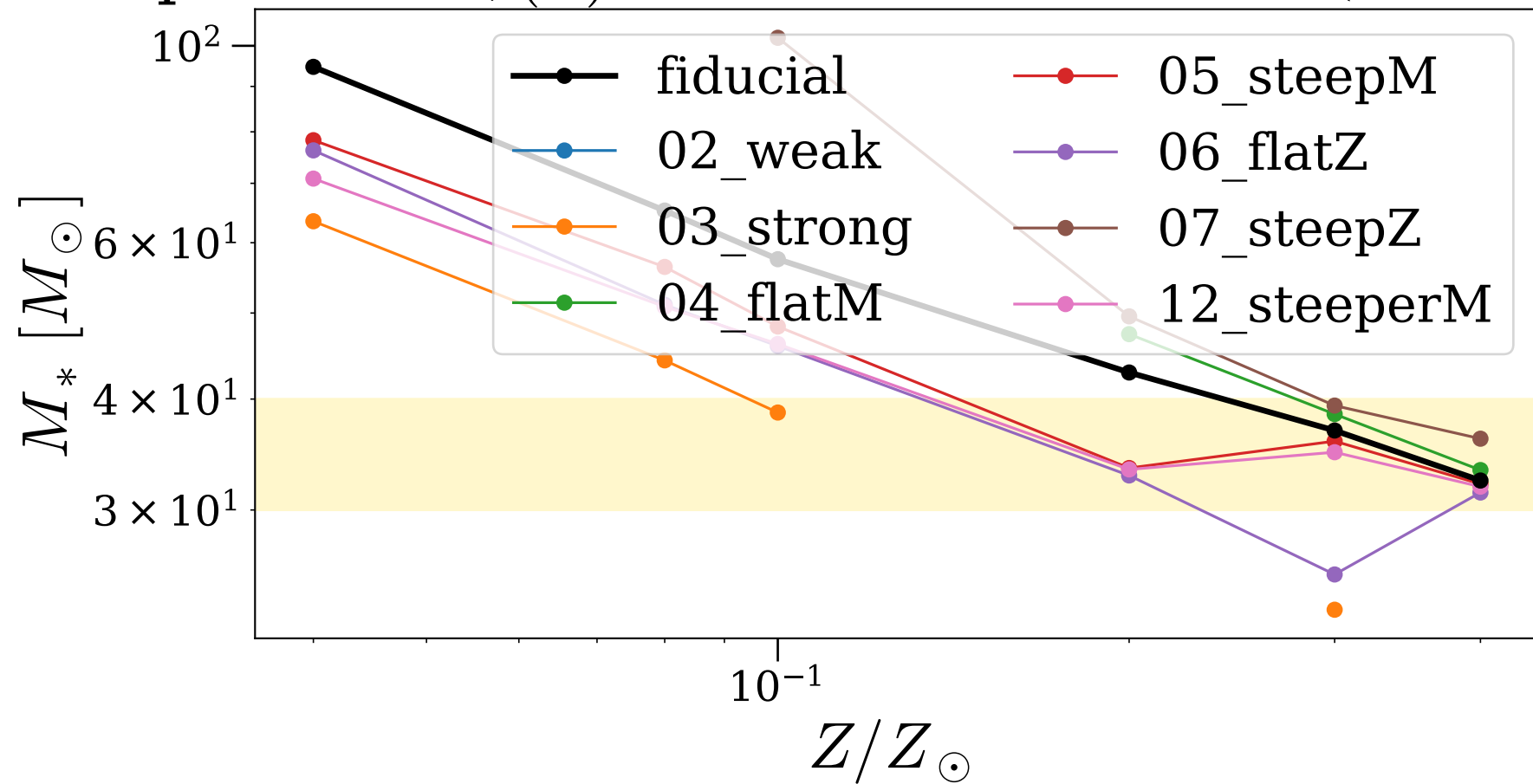
Pile-up locus M_*(Z) across wind variants ( \Phi = 0 at \theta = 0.5 )
