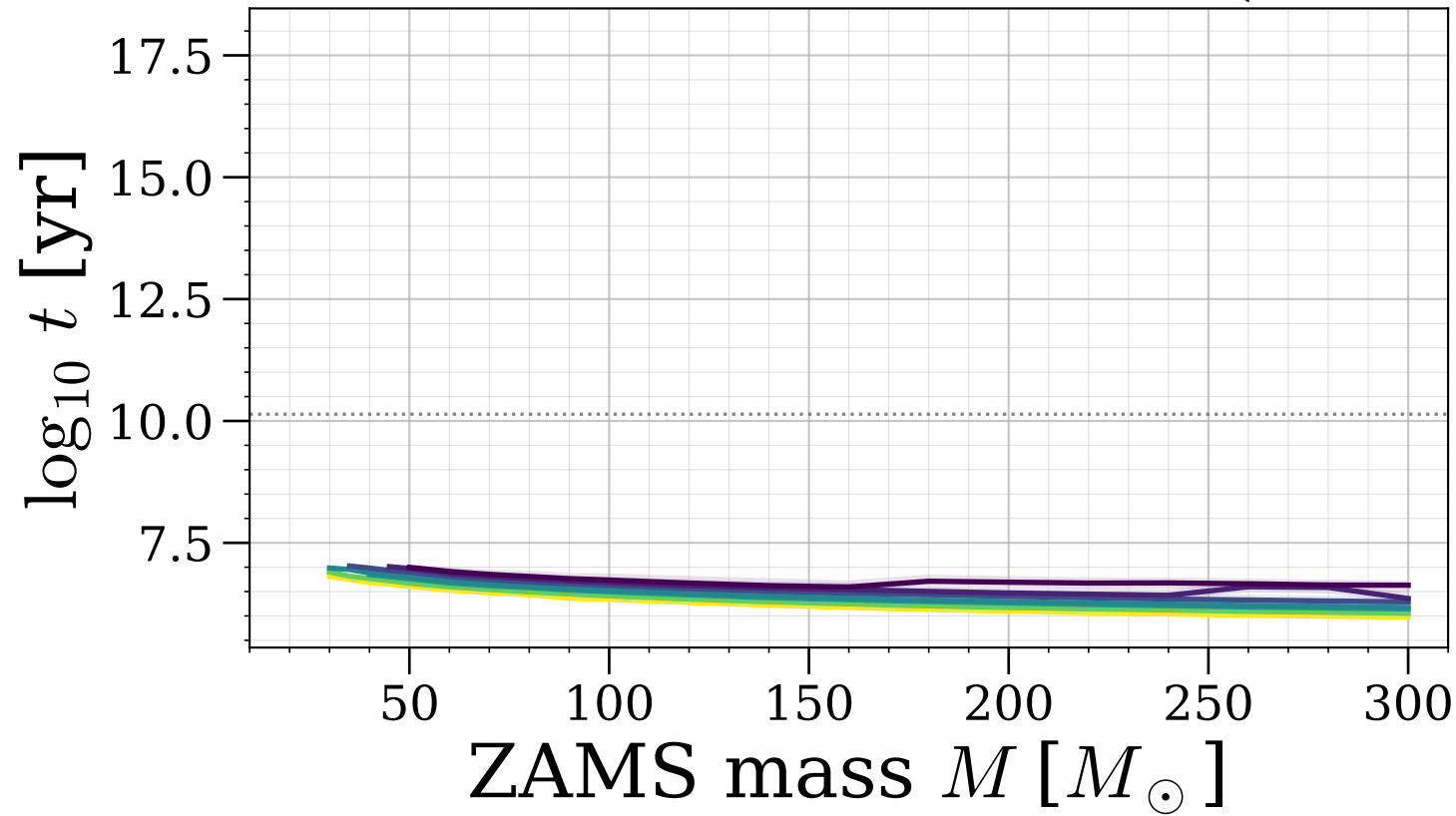
Peters time from ZAMS radii ( a = 2^{1/3}a_0 ) Actual delay time t_d (full binary evolution)
