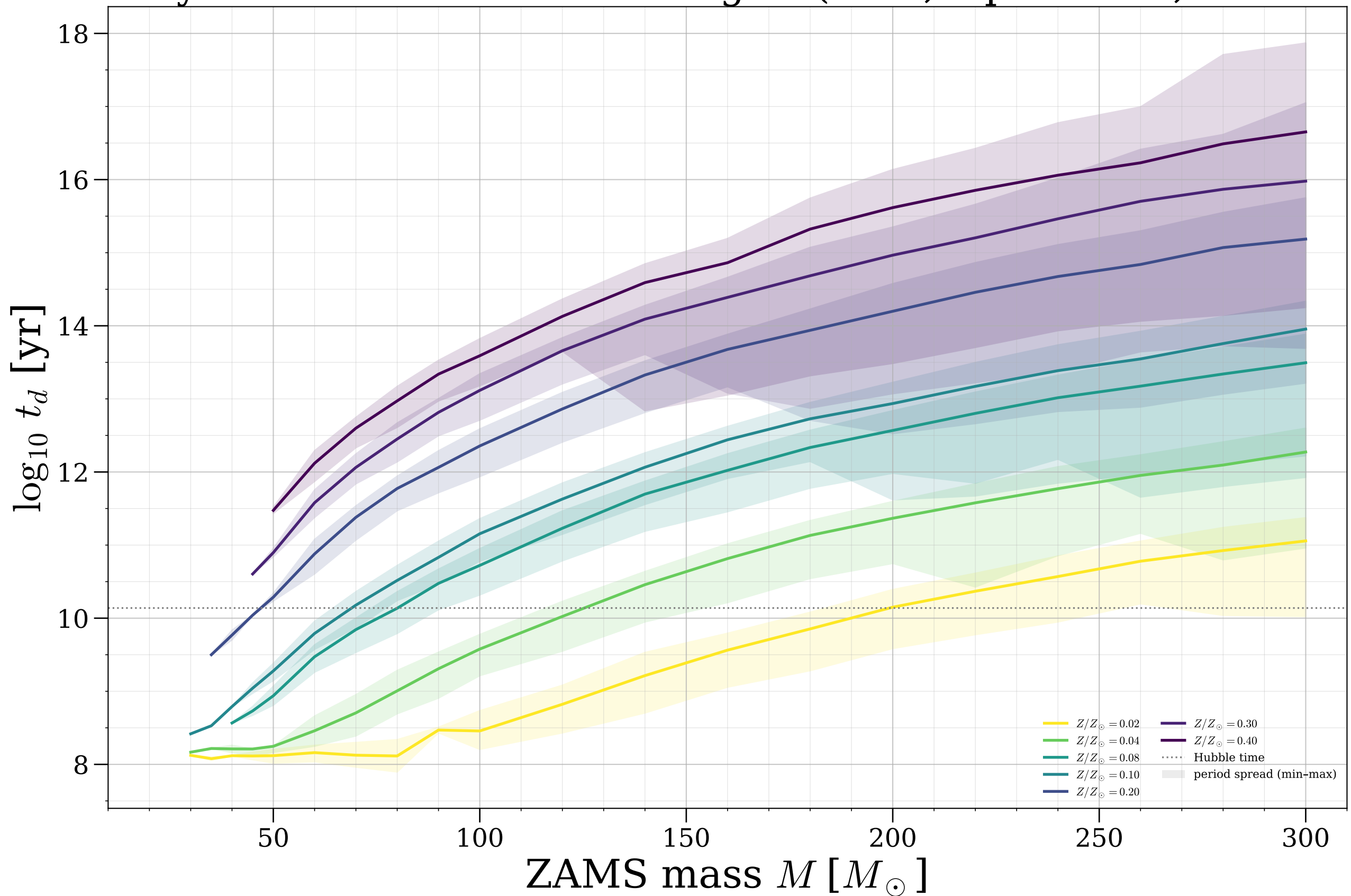
Delay time from MESA fiducial grid (CHE, equal mass, circular)
