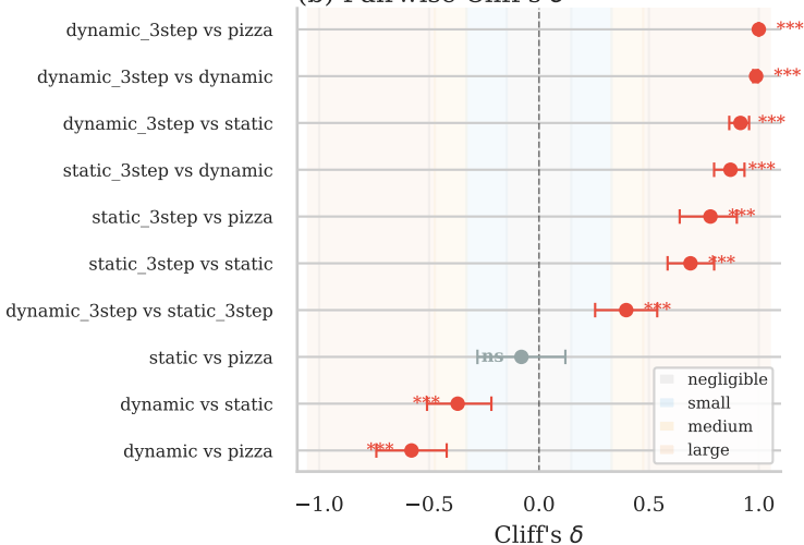
(b) Pairwise Cliff's \delta
