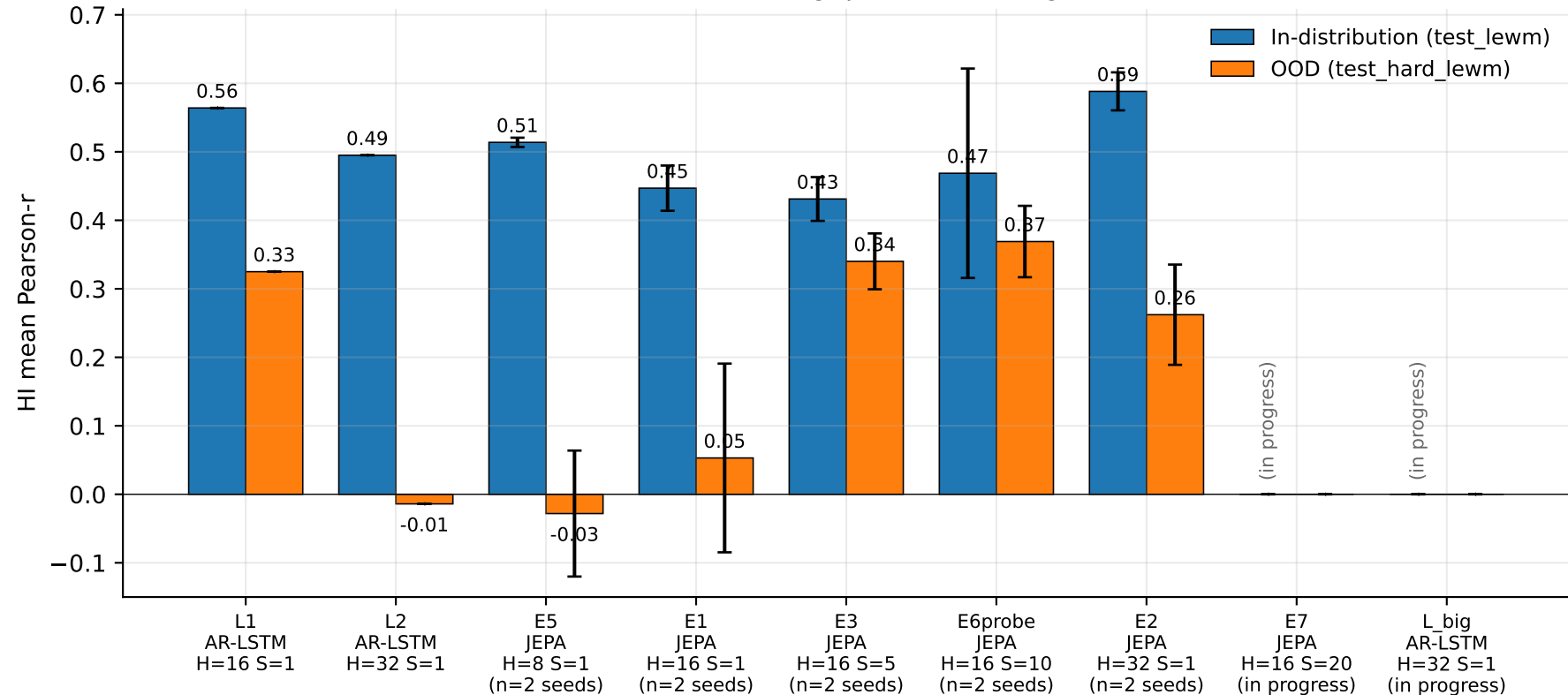
Encoder representation quality — multi-seed mean \pm std (where available)
