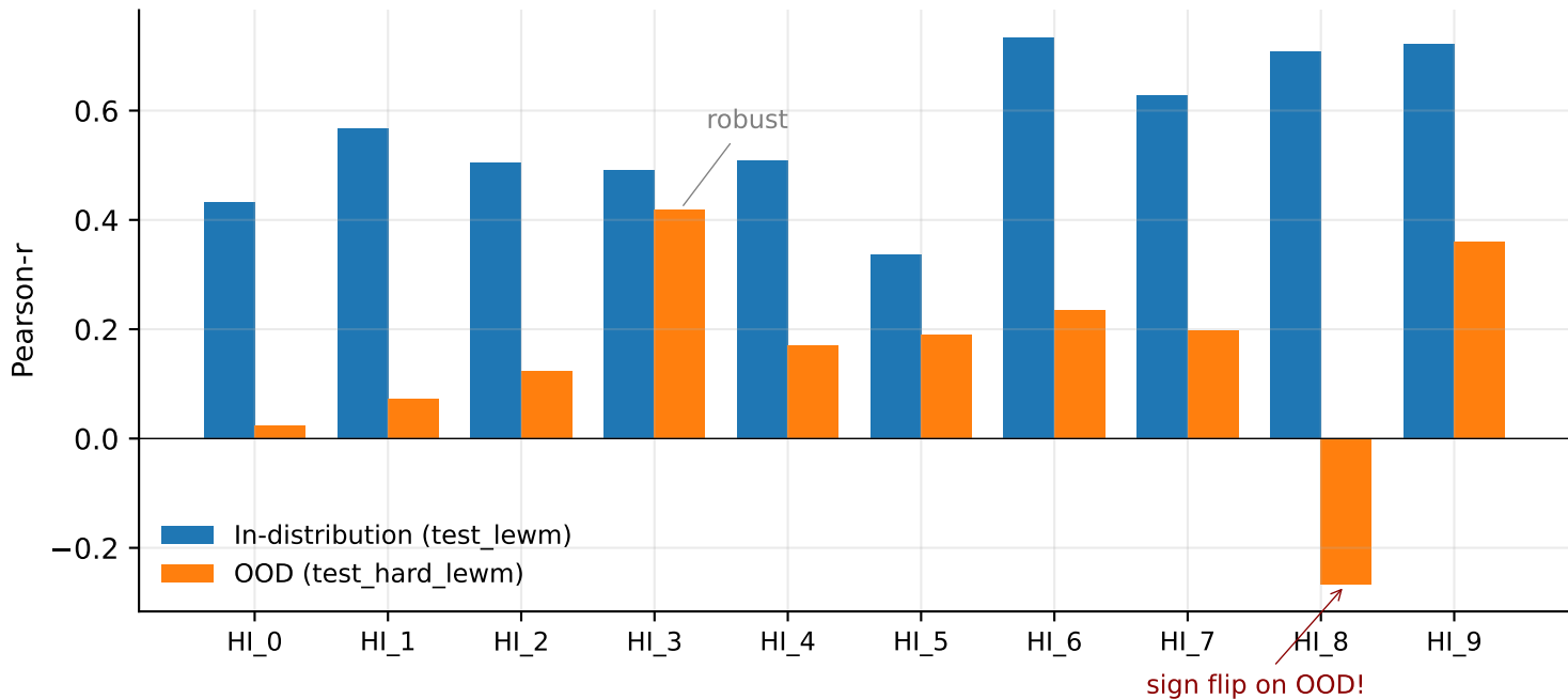
E1 (JEPA, H=16): per-HI Pearson — robust vs distribution-shift-sensitive components
