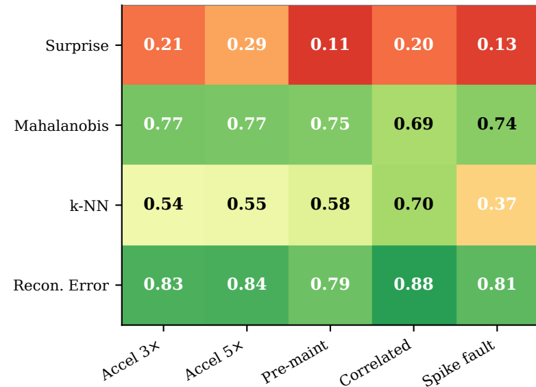
Task 4 — OOD Detection AUC-ROC
