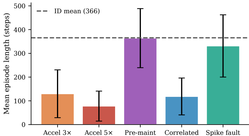
Mean OOD Episode Length (from eval run, n=50)
