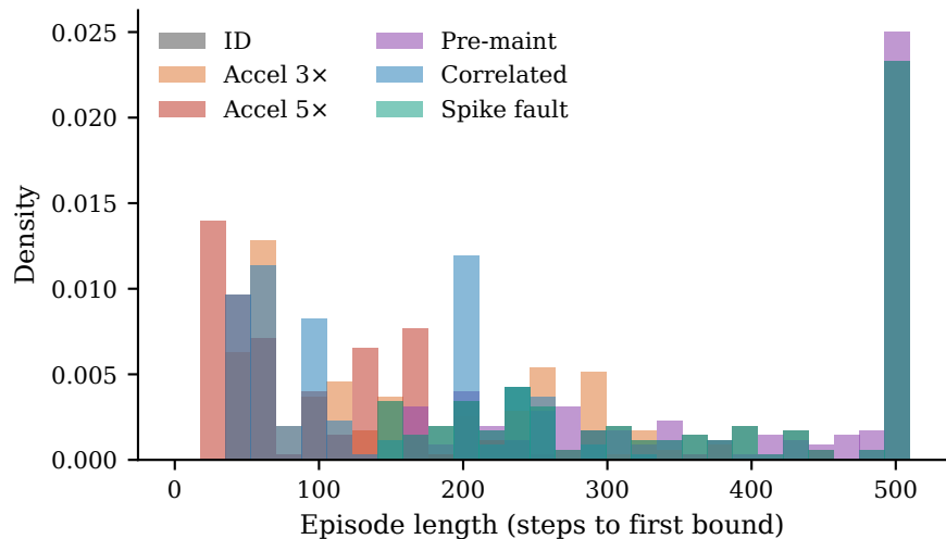
Episode Length Distribution
