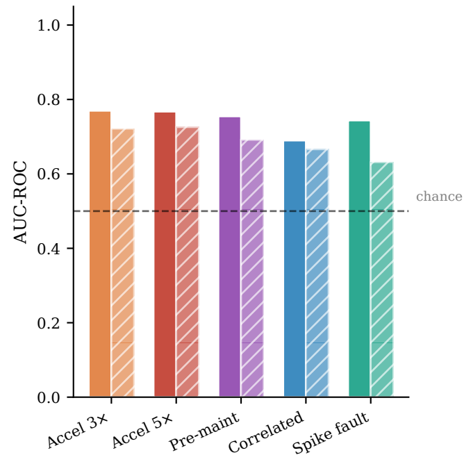
Mahalanobis detector
