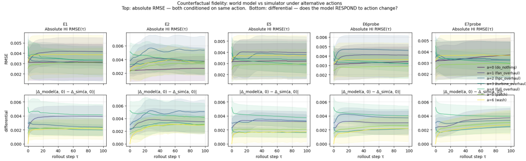
Figure 11: Counterfactual fidelity per checkpoint and per action. Top row: absolute HI RMSE between world model and simulator under the same overridden action a . Bottom row: differential |\Delta_{\text{model}}(a, 0) - \Delta_{\text{sim}}(a, 0)| , isolating the response to the action change against the do nothing baseline.
