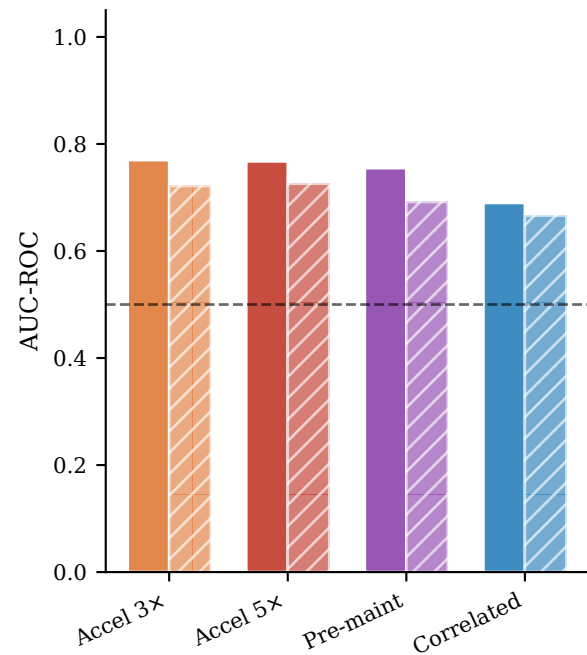
Mahalanobis detector
