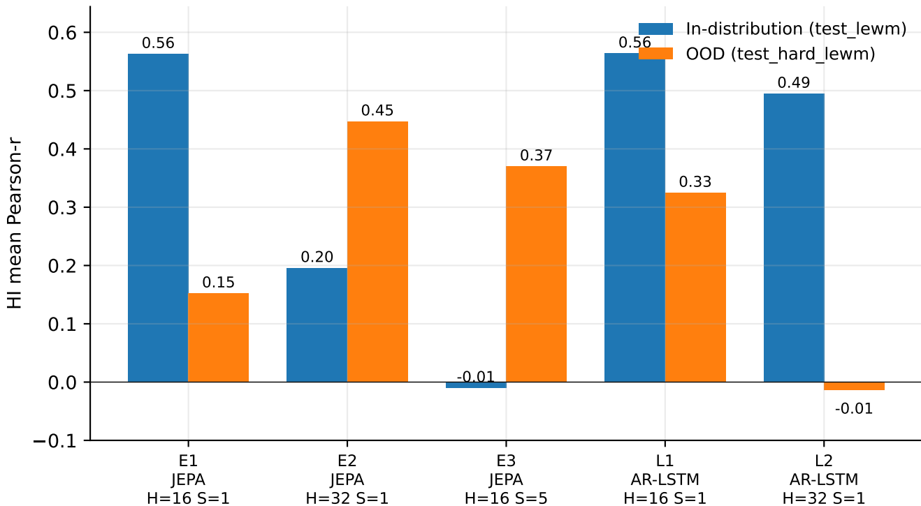
Encoder representation quality across configurations and architectures
