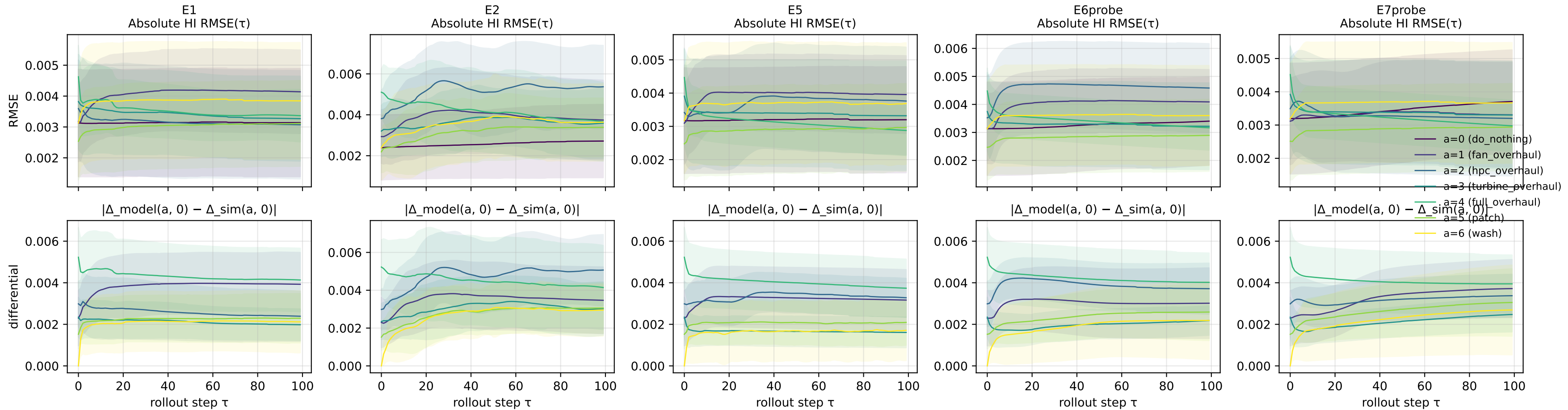
Counterfactual fidelity: world model vs simulator under alternative actions Top: absolute RMSE — both conditioned on same action. Bottom: differential — does the model RESPOND to action change?
