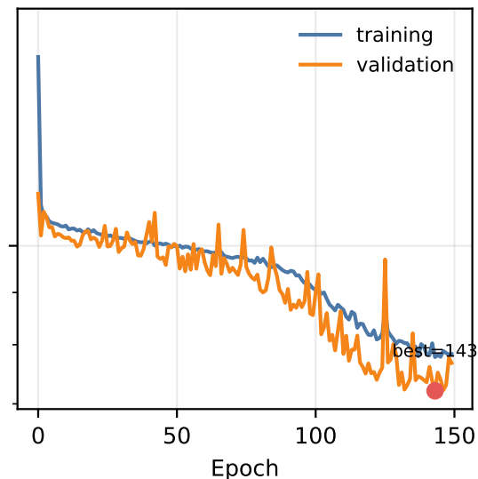
GCNM stage 2
