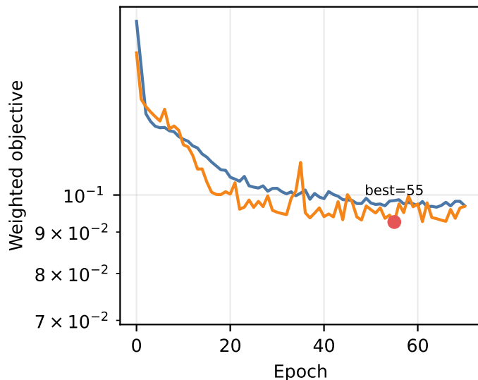
GCNM stage 1
