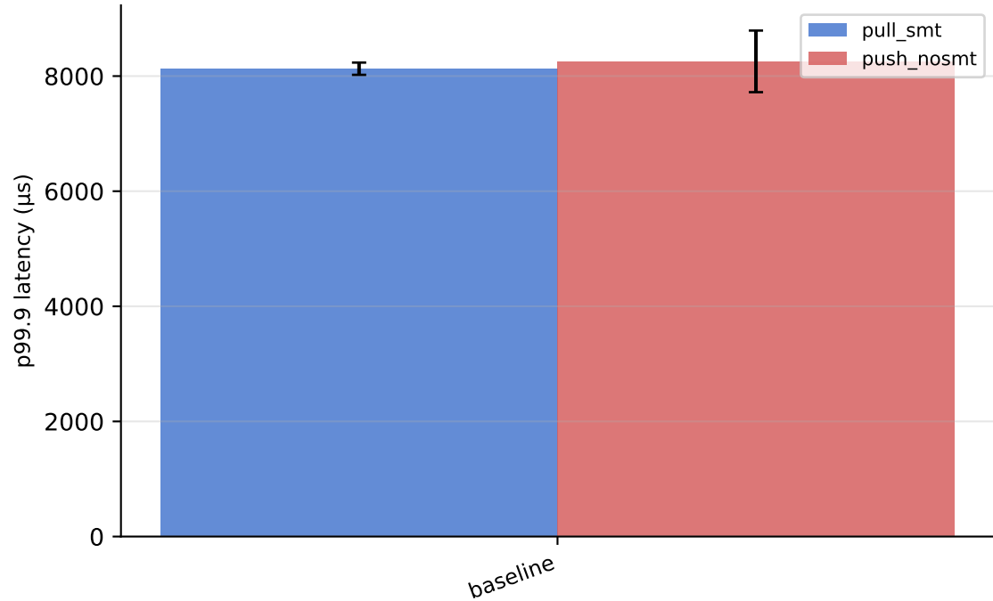
schbench — p99.9 Wakeup Latency
