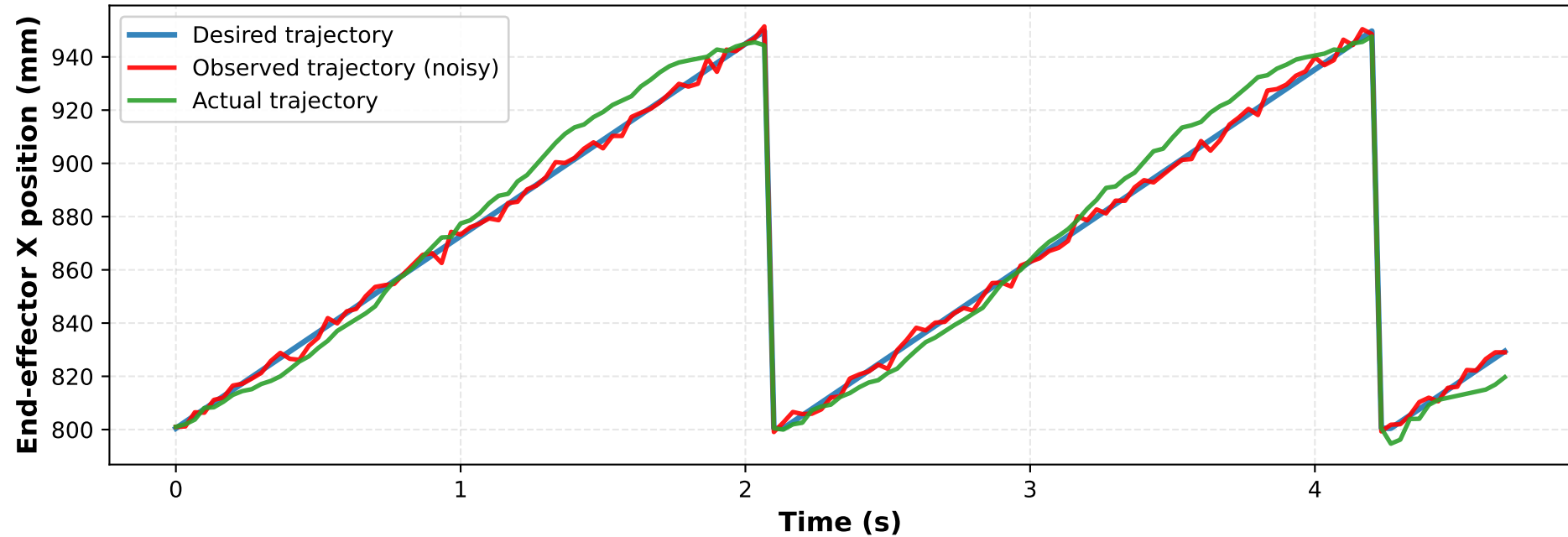
Trajectory Tracking on X-axis
