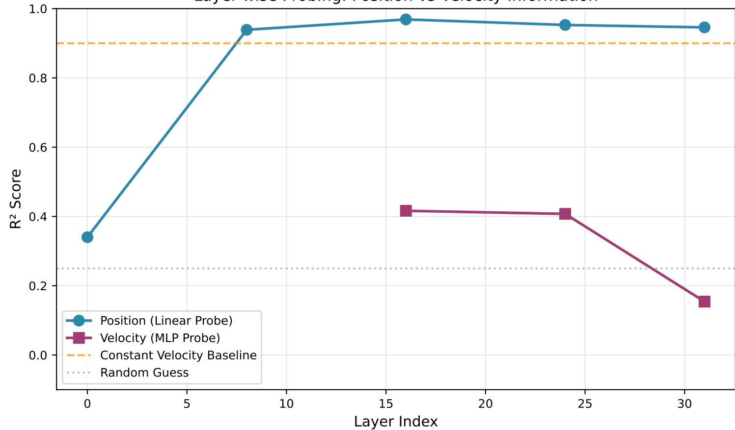
Layer-wise Probing: Position vs Velocity Information
