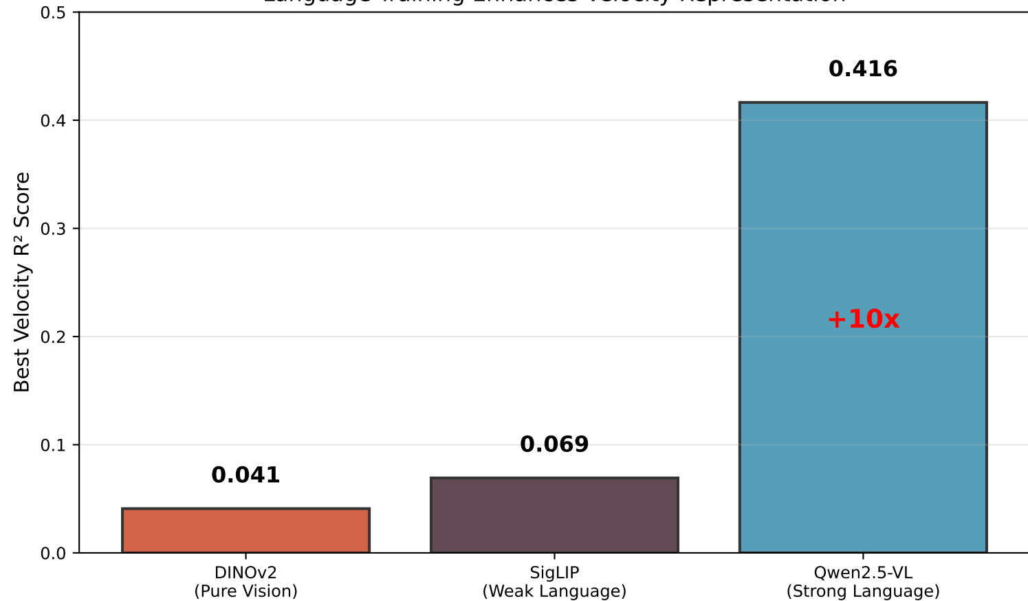
Language Training Enhances Velocity Representation
