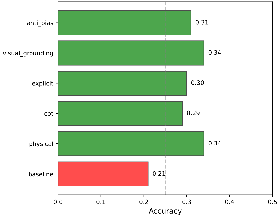
Prompt Engineering Improves Accuracy
