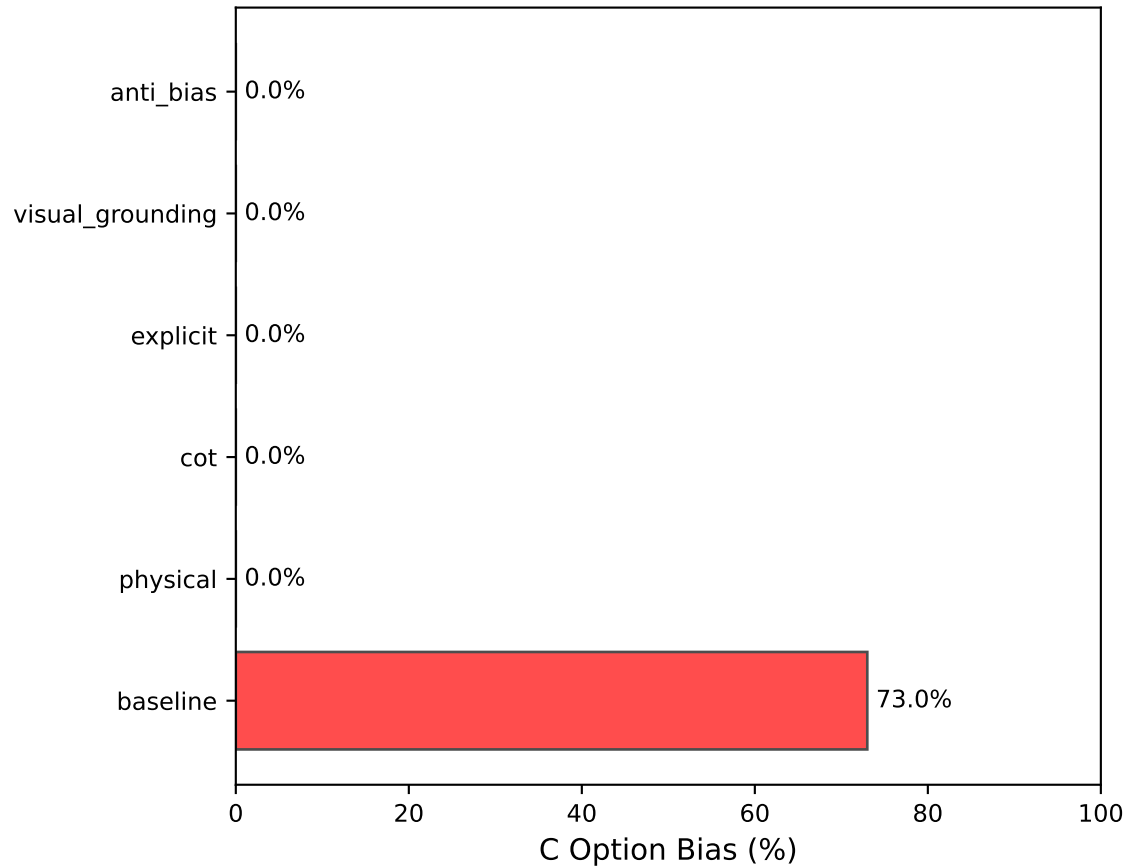
Prompt Engineering Eliminates Bias
