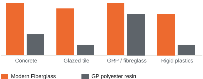
RELATIVE ADHESION BY SUBSTRATE (comparative, 0–5)
