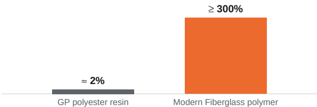
FLEXIBILITY — ELONGATION AT BREAK (typical values)
