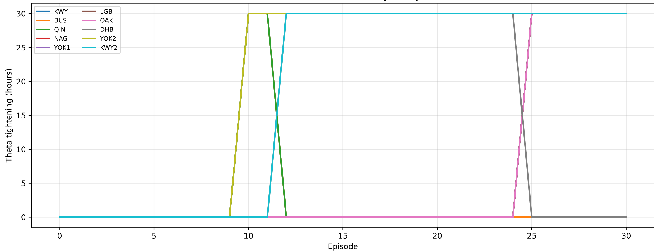
Fleet Theta Evolution — Spsa Update
