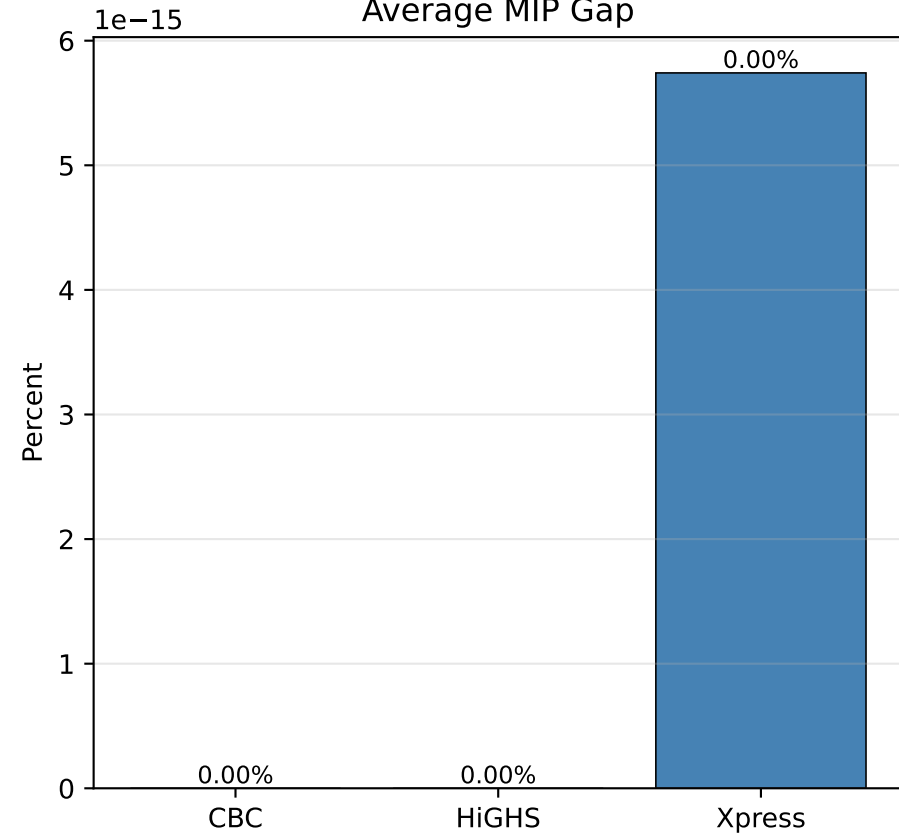
Average MIP Gap
