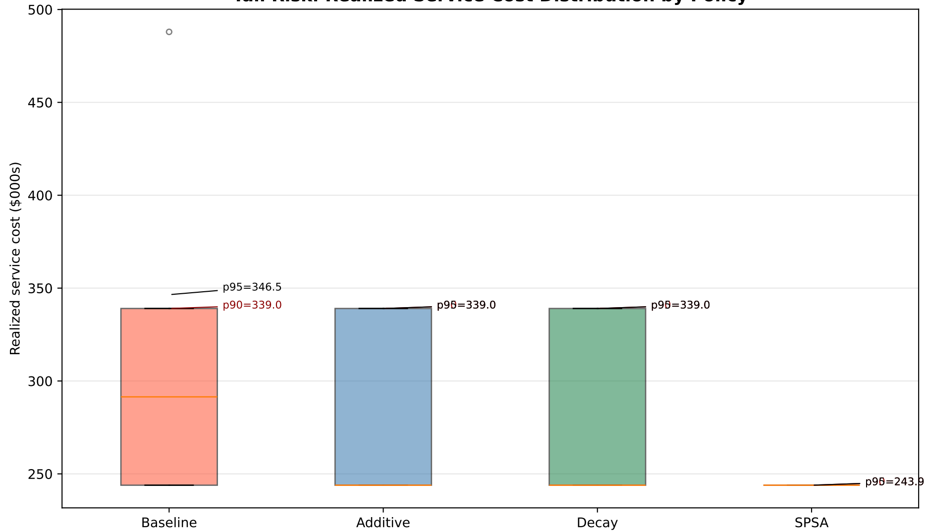
Tail Risk: Realized Service Cost Distribution by Policy
