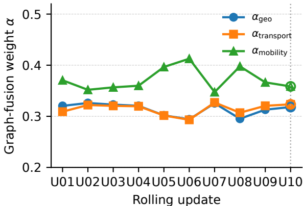
Edinburgh graph-fusion \alpha
