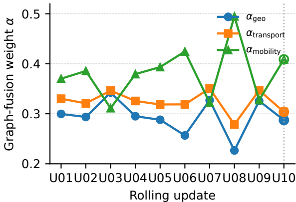
Glasgow graph-fusion \alpha
