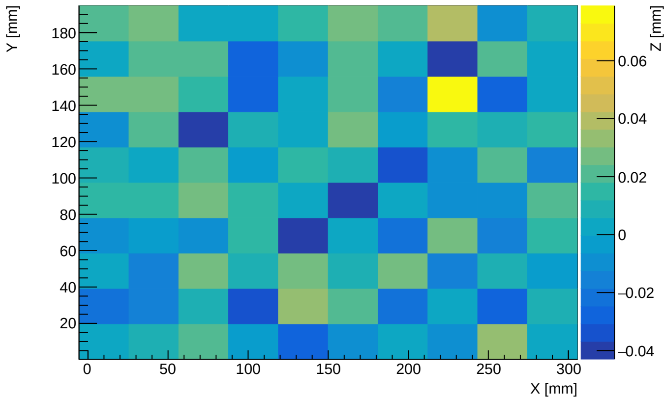
Flatness Map
