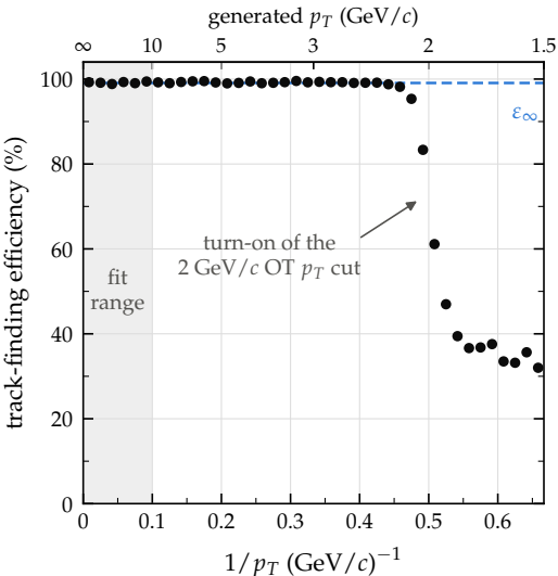
(a) whole sample
