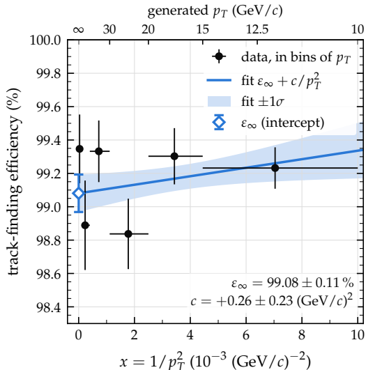
(b) the fit, p_T > 10 \text{ GeV}/c
