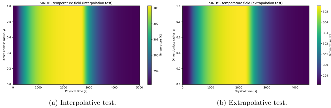
Figure 33: Spatially uniform temperature maps reconstructed by integrating the sparse thermal equation identified through SINDYc.
