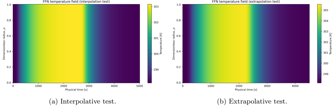
Figure 34: Spatially uniform temperature maps reconstructed through the FFN thermal rollout.
