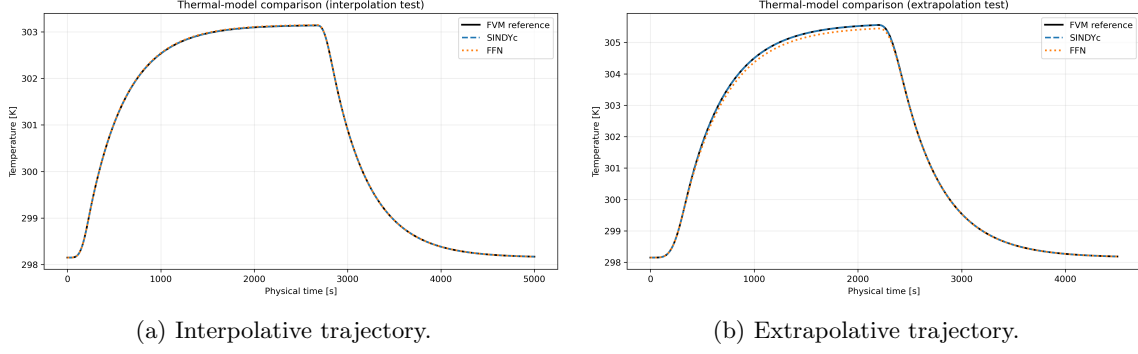
Figure 32: Temperature trajectories reconstructed by SINDYc and the FFN compared with the full-reference thermal state.
