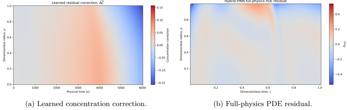
Figure 37: Space–time maps of the Hybrid-PINN residual correction and its a posteriori full-physics differential residual.
