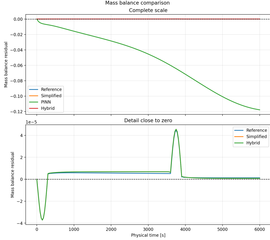
Figure 30: Mass-balance comparison. Each model is evaluated with the boundary flux belonging to its own formulation.
