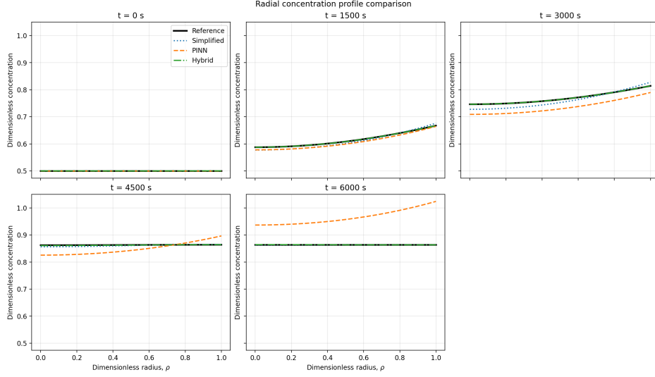
Figure 29: Radial concentration profiles at selected physical times.
