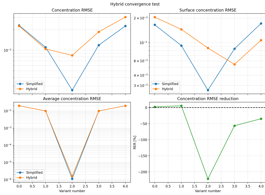
Figure 31: Convergence test for the frozen nominal correction under changes in simplified initial concentration and diffusivity.
