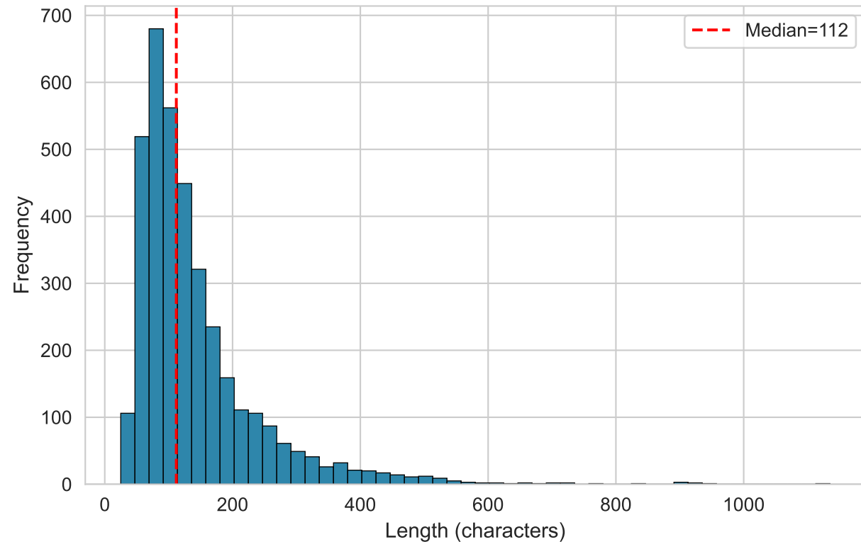
Length distribution (characters)
