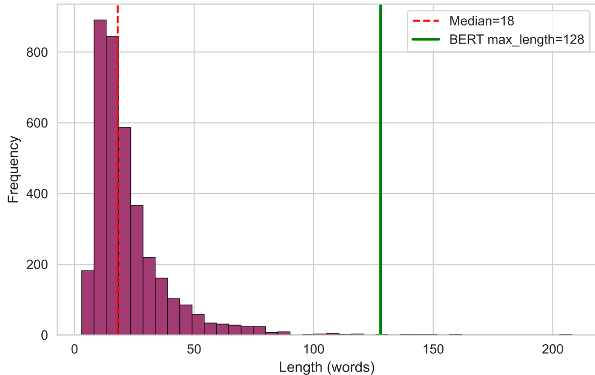
Length distribution (words)
