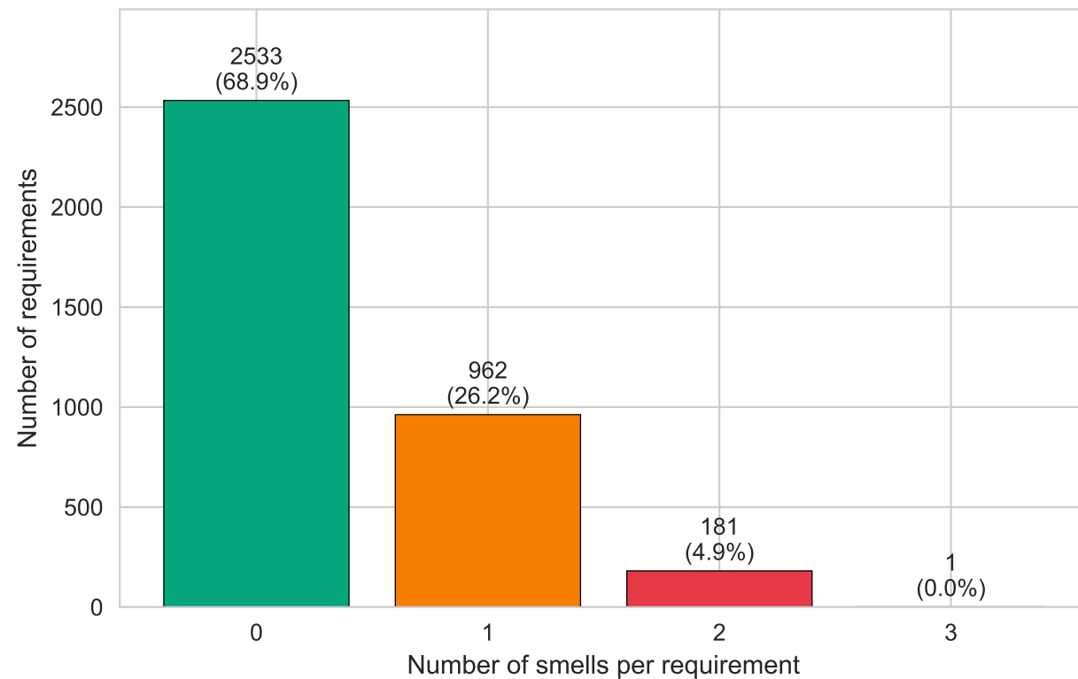
Number of smells distribution
